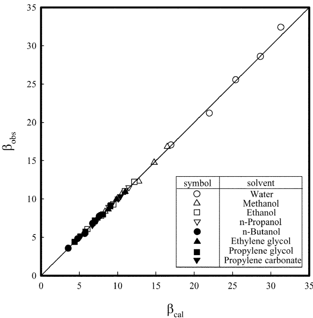
Fig. 5. Comparison of estimated enhancement factor with observed for CO 2 absorption into solvent of AMP.
