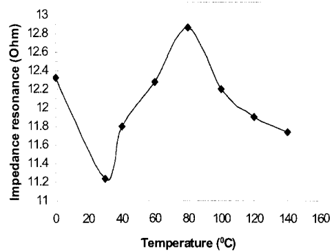
Fig. 5. Impedance resonance as a function of temperature
