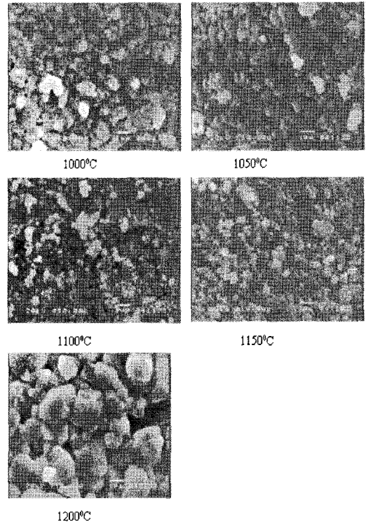
Fig. 3 SEM morphology of PZT ceramic calcined at 900°C for 4h and sintered at 1000°C, 1050°C, 1100°C, 1150°C, 1200°C for 2h
