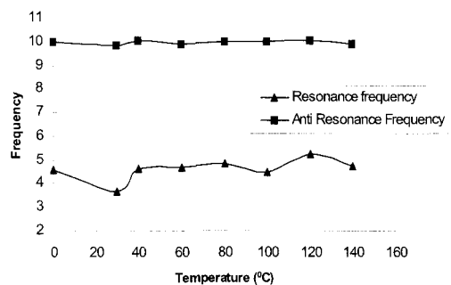
Fig. 6. Resonance frequency and anti resonance frequency as a function of temperature
