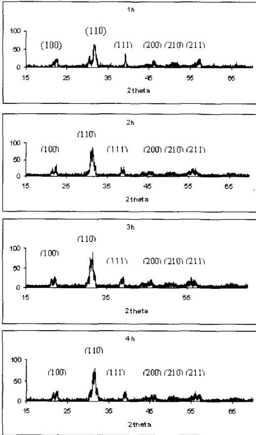
Fig. 2. X-ray diffraction patterns for PZT powders calcined at 900°C as a function of calcining time
