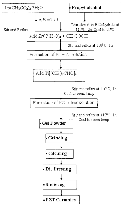
Fig. 1. Flow diagram for the preparation of PZT
