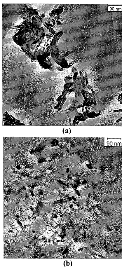
Figure 4. Transmission electron micrographs of PC/MWCNT (95/5 wt%) composites obtained by solution mixing: (a) MWCNT was untreated; (b) MWCNT was freeze-dried after treatment with H_2O_2 .
