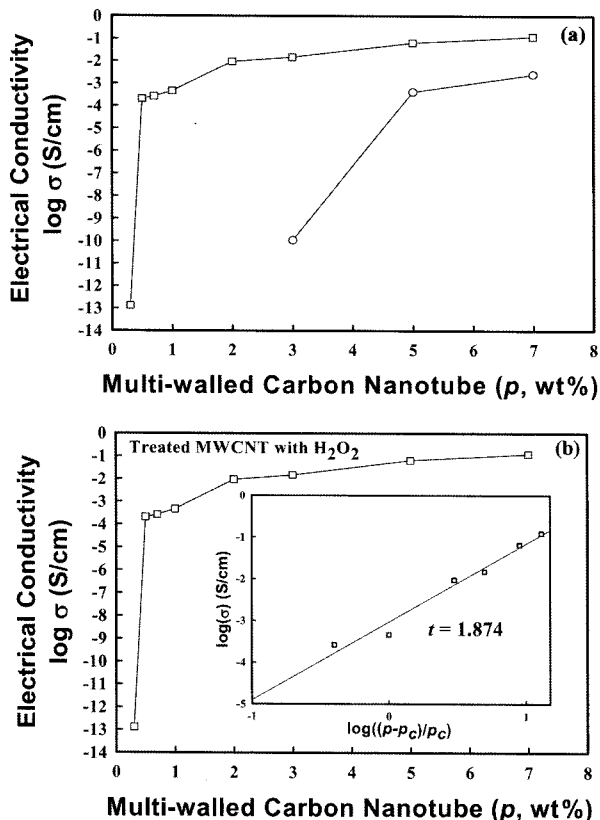
Figure 1. (a) Electrical conductivity of PC/MWCNT composites with MWCNT content: ( \circ ) MWCNT was untreated; ( \square ) MWCNT was freeze-dried after treatment with H_2O_2 . (b) The inset shows the log-log plot of electrical conductivity ( \sigma ) with (p-p_c)/p_c for p > p_c .
