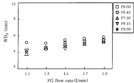
Fig. 10 Relationship between PG flow rate and WB_B at each position
