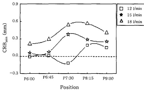
Fig. 17 Relationship between position and CRB min at each SG flow rate
