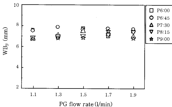
Fig. 9 Relationship between PG flow rate and WB_F at each position
