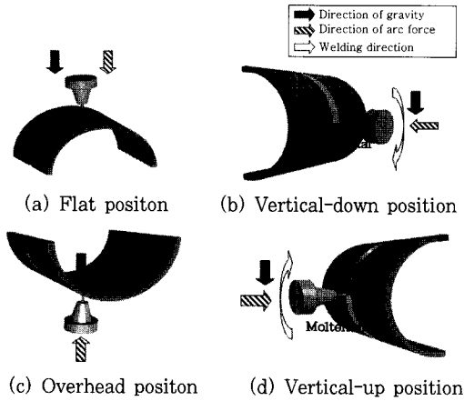
Fig. 2 Direction of forces at each position
