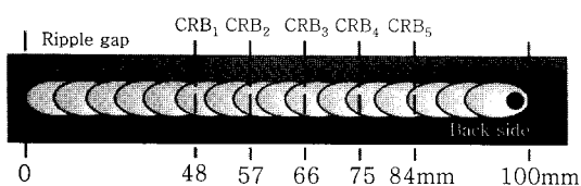
Fig. 6 Schematic of measurement interval for CRB
