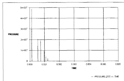
Fig. 16 Pressure curve for bird strike.
