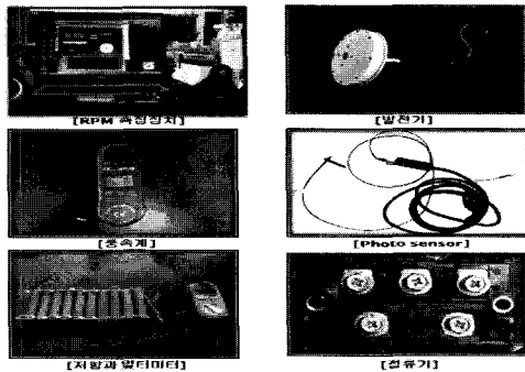
Fig. 27 Equipment for the blade performance test
