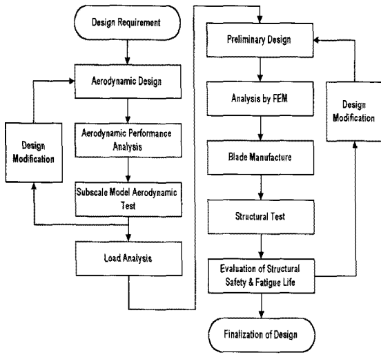
Fig. 1 Flow of aerodynamic and structural design.
