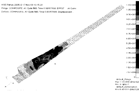
Fig. 18 Stress result of the bird strike analysis.
