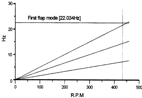
Fig. 10 Campbell diagram for load case 2.
