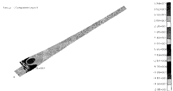
Fig. 9 Stress analysis result for cyclic load.
