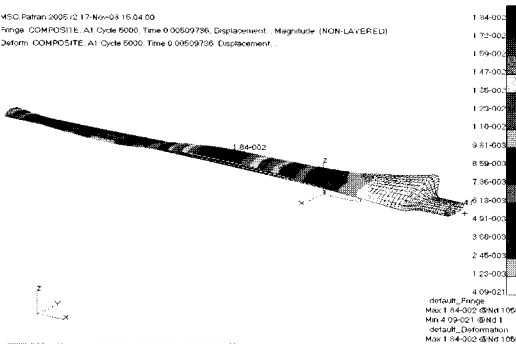
Fig. 19 Displacement result of the bird strike analysis.
