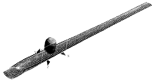
Fig. 14 Modeling for bird strike.
