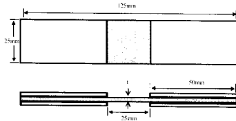
Fig. 3 Specimens for the compression-compression fatigue test.
