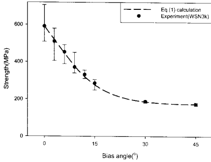
Fig. 7 Compressive strength of bias specimens for carbon/epoxy composites.
