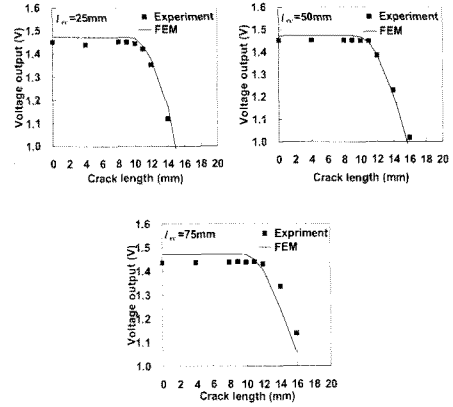
Fig. 8 Measured and calculated electric voltage output of unidirectional carbon fiber epoxy composites by the electric potential method with the bridge circuit concept with respect to the distance ( l_c ) between the electrode and crack.
