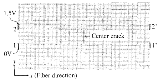
Fig. 4 Finite element model for analyses of electric potential changes with the bridge circuit concept.
