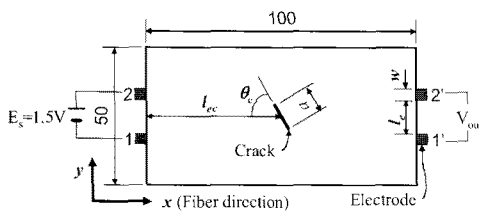
Fig. 3 Composite specimens for the crack detection by the electric potential method with the bridge circuit concept(unit in mm).
