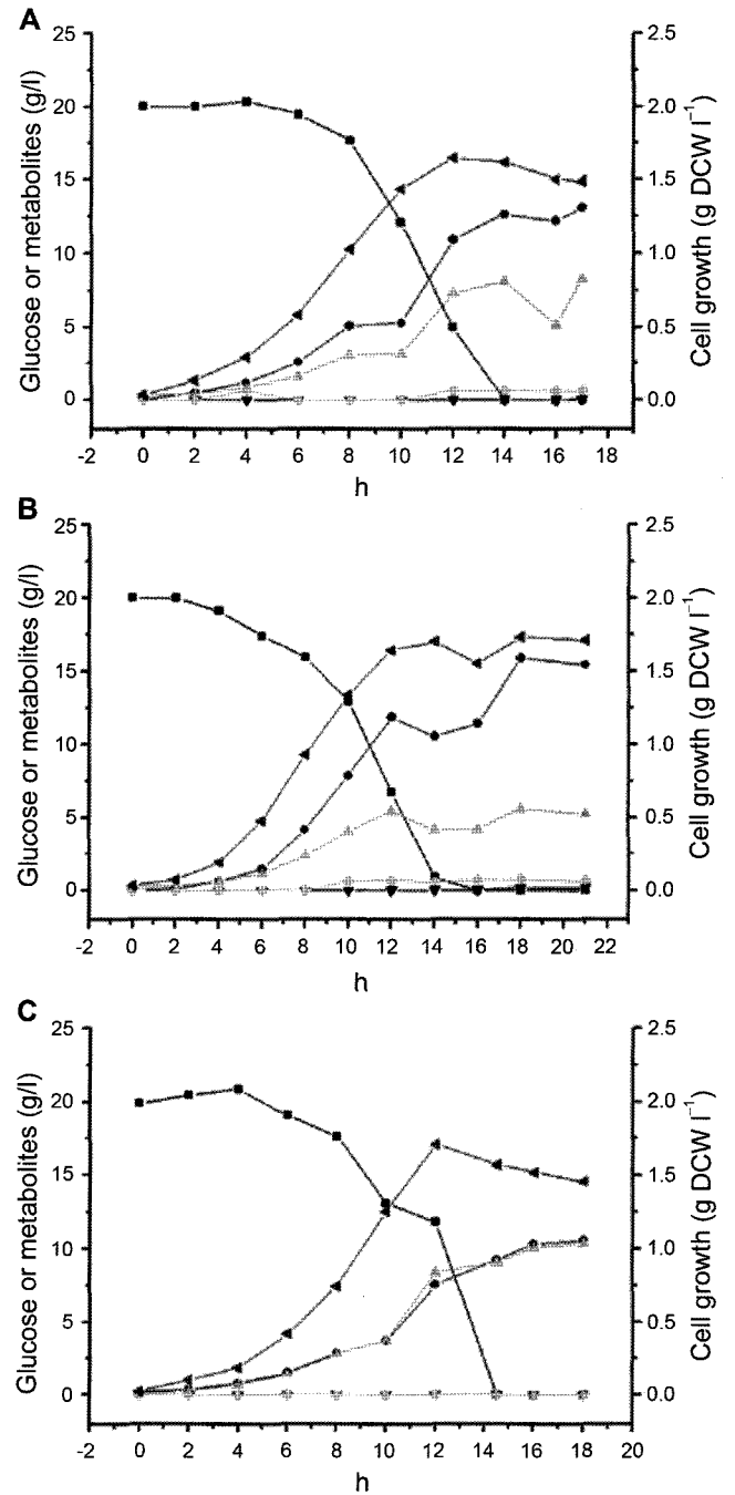
Fig. 2. Effect of agitation speed on succinic acid production at a working volume of 7.0 l; (A) 75 rpm, (B) 150 rpm, (C) 300 rpm. ●, Succinic acid; ■, glucose; ▲, pyruvic acid; ▼, formic acid; ◆, acetic acid; ◀, cell growth.
