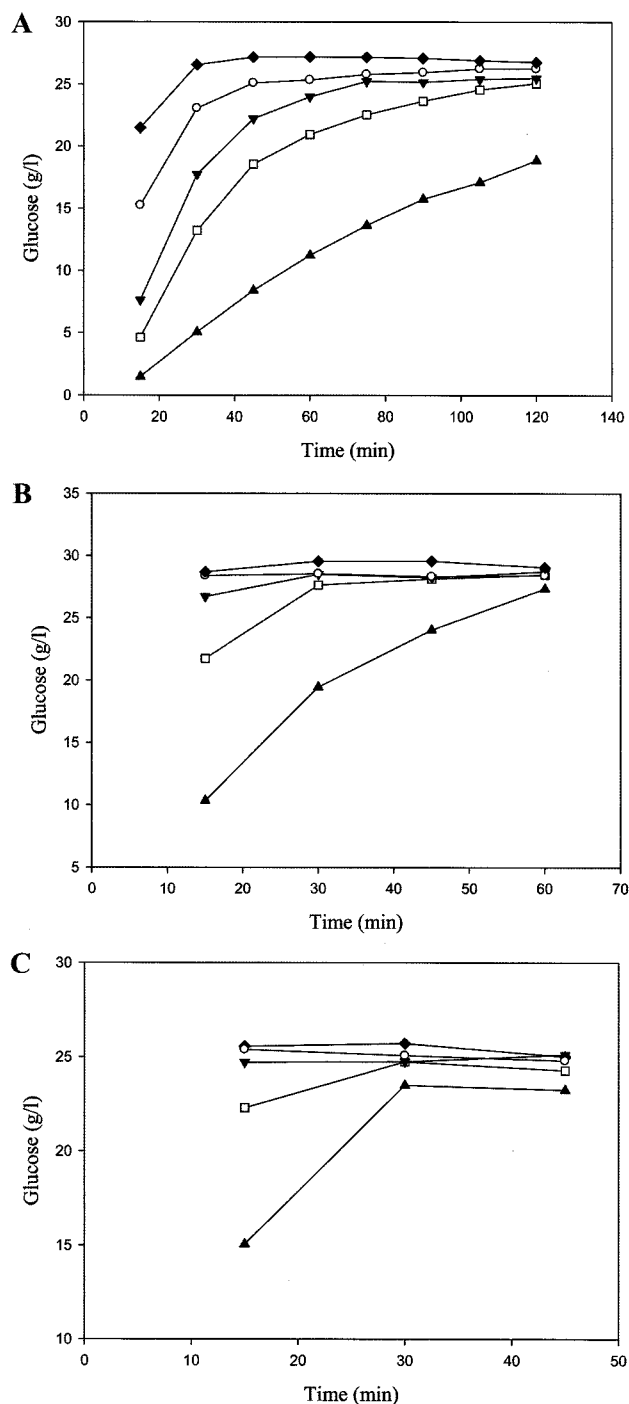
Fig. 3. Glucose released by hydrothermal dilute acid pretreatment under different conditions.
