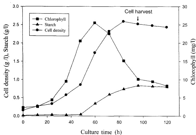
Fig. 2. Cell growth, chlorophyll content, and starch accumulation in the pH-stat fed-batch culture of C. reinhardtii UTEX 90 by feeding 1.0 M acetic acid under continuous illumination ( 450 \mu\text{E}/\text{m}^2/\text{s} ), using a 2.5-l photobioreactor.
