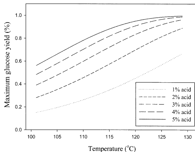
Fig. 5. Predicted maximum release of glucose as a function of temperature and pH.
