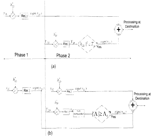
Fig. 3. Data sequence of select relaying. (a) Select relaying protocol in [2] (b) our proposed protocol
