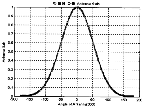
(c) Wide beam pattern
