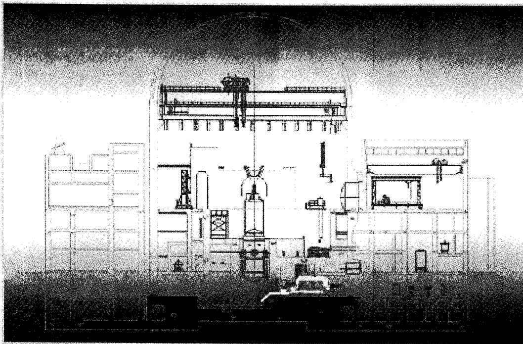
Fig. 8. The Common Basemat of the RCB and the AB
