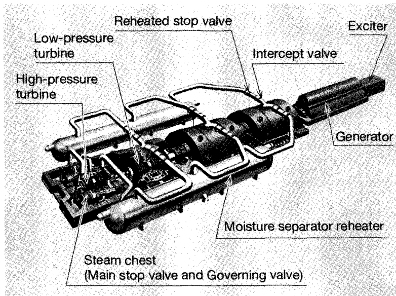
Fig. 8. Large-capacity, High-performance Turbine Generator System
