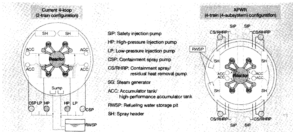
Fig. 4. Emergency Core Cooling System
