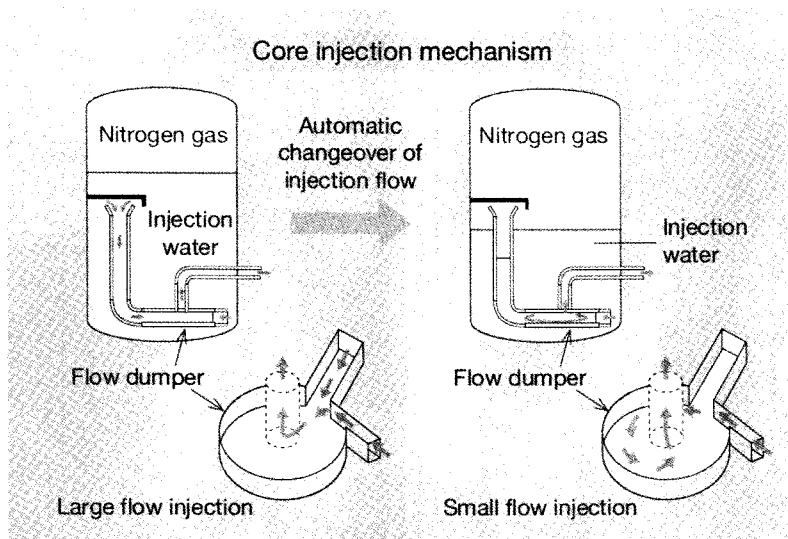
Fig. 5. High-performance Accumulator Tank
