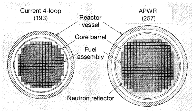
Fig. 2. Adoption of Large Core
