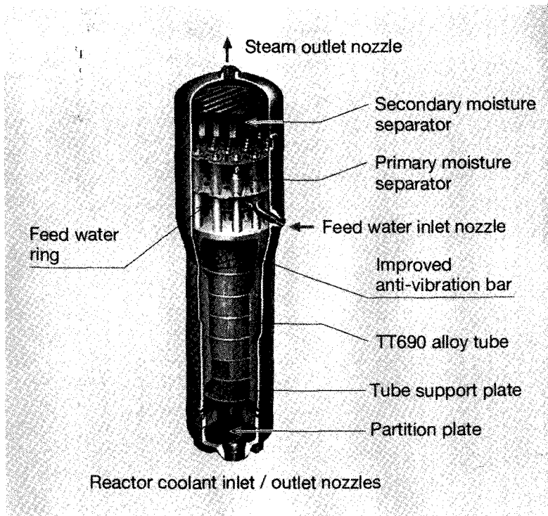
Fig. 7. High-performance, Compact Steam Generator
