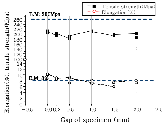
Fig. 12 Tensile strength and elongation of FSW with gap
