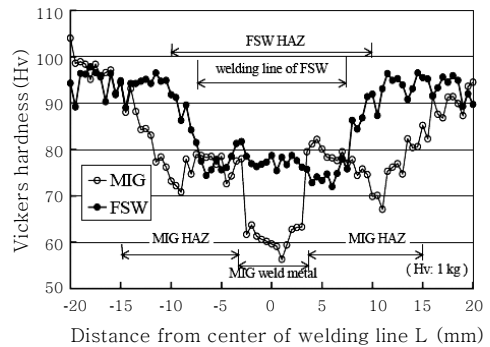
Fig. 1 Comparison of FSW and MIG (A6N01-T5)
