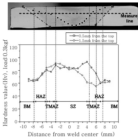
Fig. 6 Cross section and hardness in FSW
