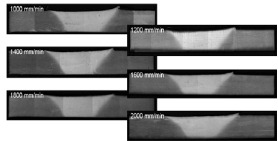
(b) Cross section
