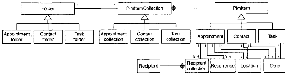
Figure 3. The Pocket Outlook Object Model.
