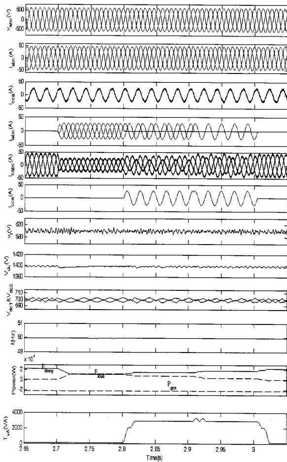
Fig. 4 Performance of the controller under application of balanced/unbalanced linear loads
