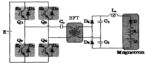
Fig. 3 High frequency link series resonant DC-DC converter(Circuit 1)
