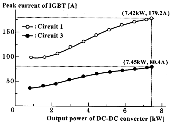
Fig. 12 Comparison of peak values of current flowing through IGBT
