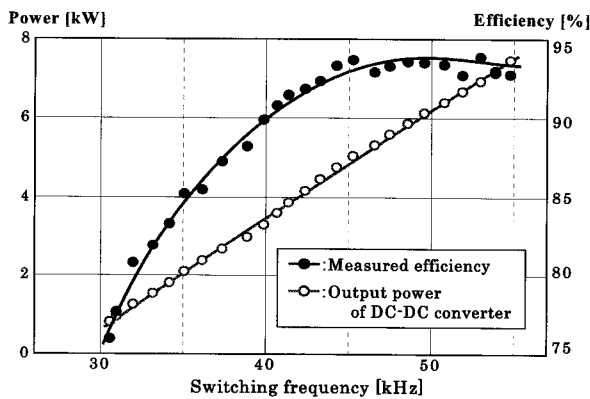
Fig. 13 Output power and measured efficiency vs. switching frequency characteristics with newly design specification of circuit 2
