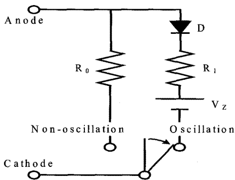
Fig. 2 Electrical equivalent circuit model of magnetron
