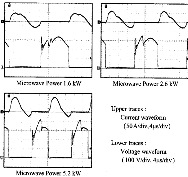
Fig. 11 Experimental voltage and current waveforms of Q1 (Circuit 3)
