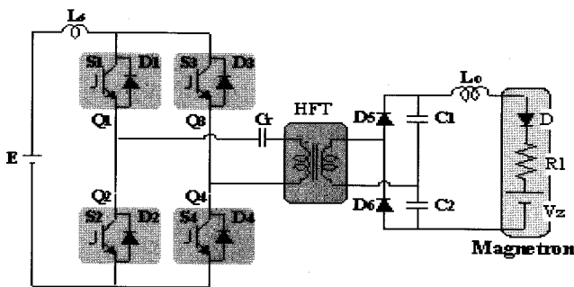
Fig. 6 Proposed soft switching DC-DC power converter (Circuit 2)
