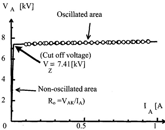
Fig. 1 Experimental characteristics of magnetron
