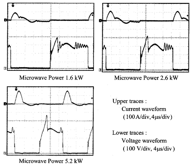
Fig. 8 Experimental voltage and current waveforms of Q1 (Circuit 2)
