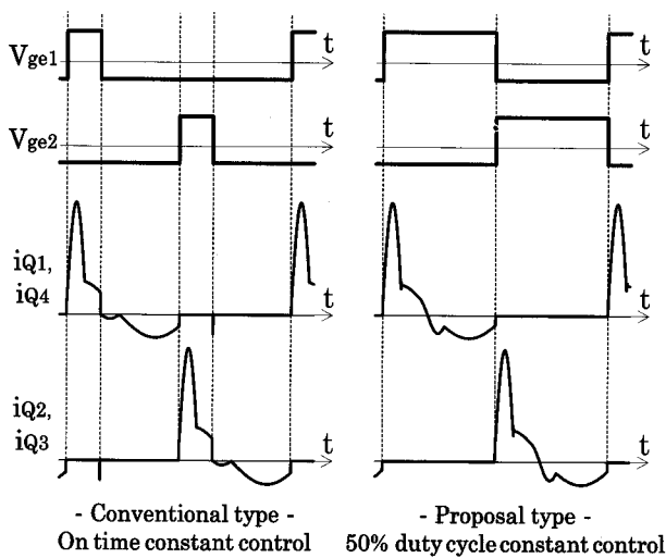
Fig. 7 50% duty cycle constant PFM control scheme
