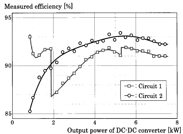
Fig. 10 Comparison of power conversion efficiency vs. output power characteristics for two converter topologies
