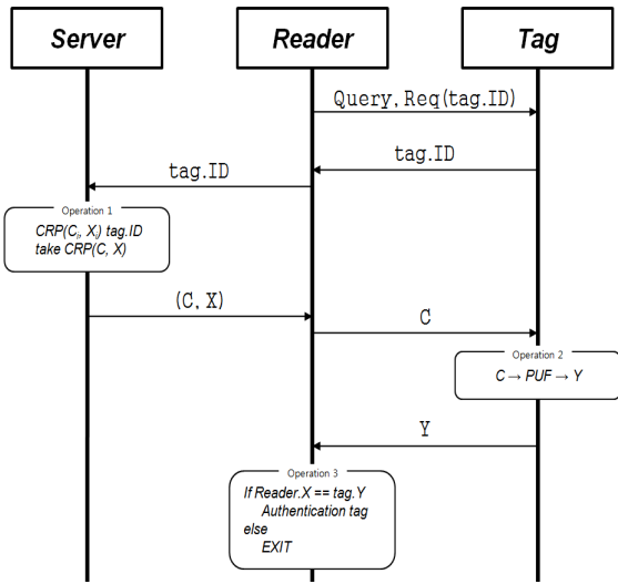
(그림 5) PUFs and Public-Key Cryptography for RFID-Tags
