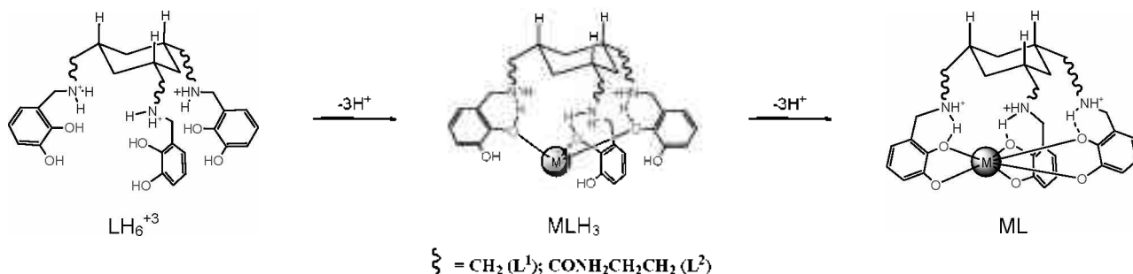
Figure 5. Possible coordination mode for ligands, L^1 and L^2 with the metal ions.
