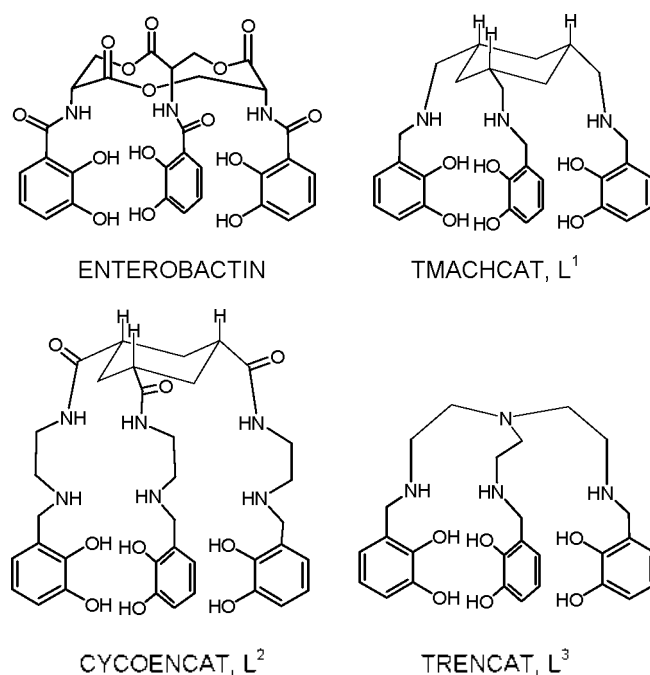
Figure 1. Molecular structure of ENTEROBACTIN, TMACHCAT (L 1 ), CYCOENCAT (L 2 ) and TRENACAT (L 3 ).
