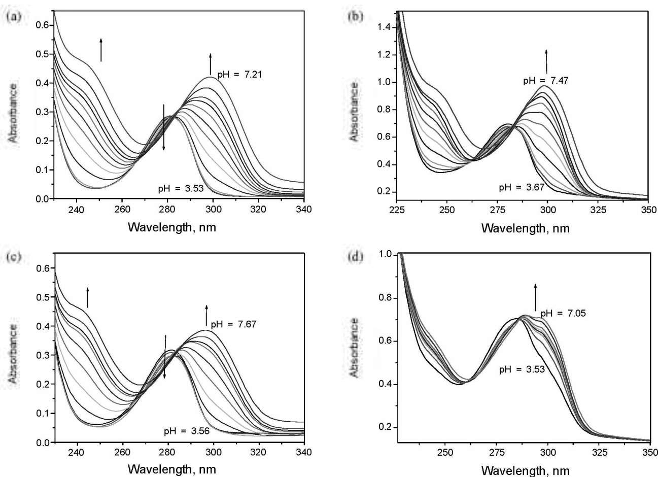
Figure 3. Experimental electronic spectra at 1:1 metal to ligand ratio for (a) GaL^1 , (b) GaL^2 , (c) InL^1 , and (d) InL^2 systems.
