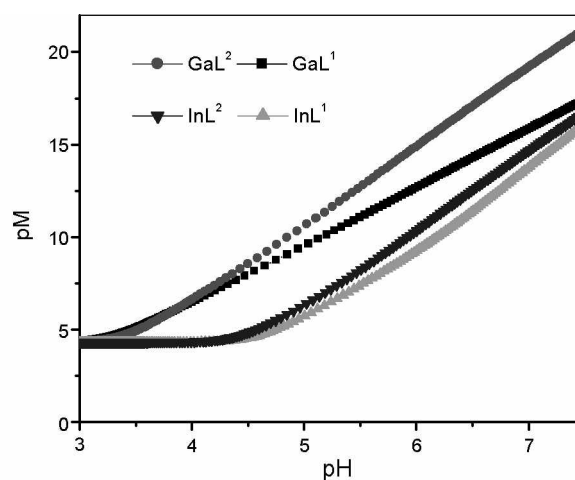
Figure 6. Plot of \text{pM} ( \text{pM} = -\log [M^{n+}] ) vs pH. \text{pM} was calculated for [L] = 5 \times 10^{-4} M ( L = L^1 or L^2 ), [M^{n+}] = 5 \times 10^{-5} M ( M^{n+} = \text{Ga}^{3+} and \text{In}^{3+} ) using the deprotonation constants of ligands L^1 and L^2 , and the complexation constants \beta_{111} .
