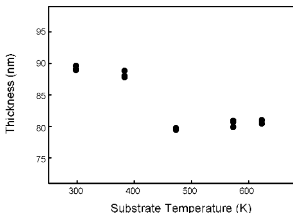
Figure 3. Thickness of zirconium oxide thin films as a function of substrate temperatures.
