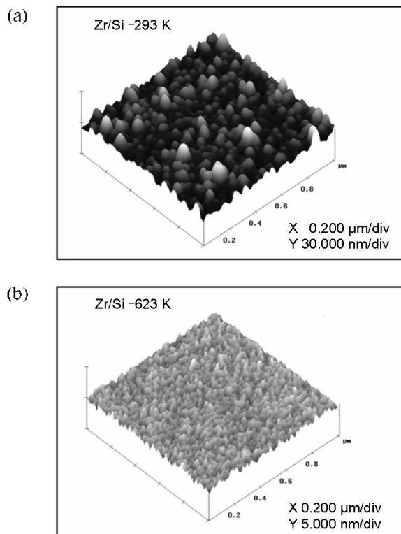
Figure 2. AFM images ( 1 \mu\text{m} \times 1 \mu\text{m} ) of zirconium oxide thin films on Si(100) with: (a) deposition at room temperature (293 K), (b) deposition and substrate heating at 623 K. Note the scale bars of y-direction: 30 nm/div. for (a) Zr/Si-293 K and 5 nm/div. for (b) Zr/Si-623 K.
