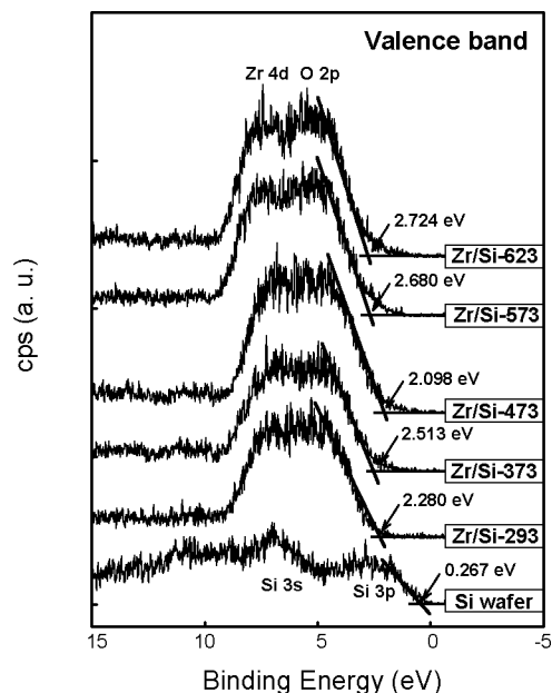
Figure 8. Valence band spectra for deposited zirconium oxide thin films on Si(100) with increased substrate temperature. The solid lines are extrapolating lines applying the least square method and the intersection of the solid lines represents the valence band maximum.
