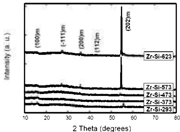
Figure 1. The XRD patterns of the zirconium oxide thin films deposited on Si(100) with different substrate temperatures in Ar/O 2 plasma ambient. The numbers in the legend box represent substrate temperatures.
