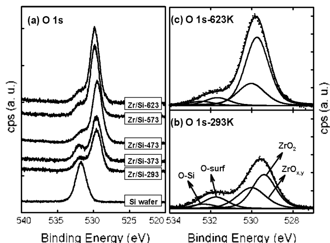
Figure 6. (a) O 1s region XP spectra of the zirconium oxide thin films on Si(100) with different substrate heating temperatures. The silicon dioxide ( \text{SiO}_2 ) peak was centered at 531.7 eV, and the zirconium oxides (O-Zr) was assigned at 529.6 eV. Deconvoluted XP spectra of the O 1s at the silicon substrate temperature was 293 K (b) and 623 K (c). The O 1s spectra were deconvoluted four oxidation states: zirconia ( \text{ZrO}_2 ), higher and lower oxidation states ( \text{ZrO}_{x,y} ), surface oxygen (O-surf), silicon dioxide (O-Si). The bottom solid lines are subtracted background by Shirley mode.
