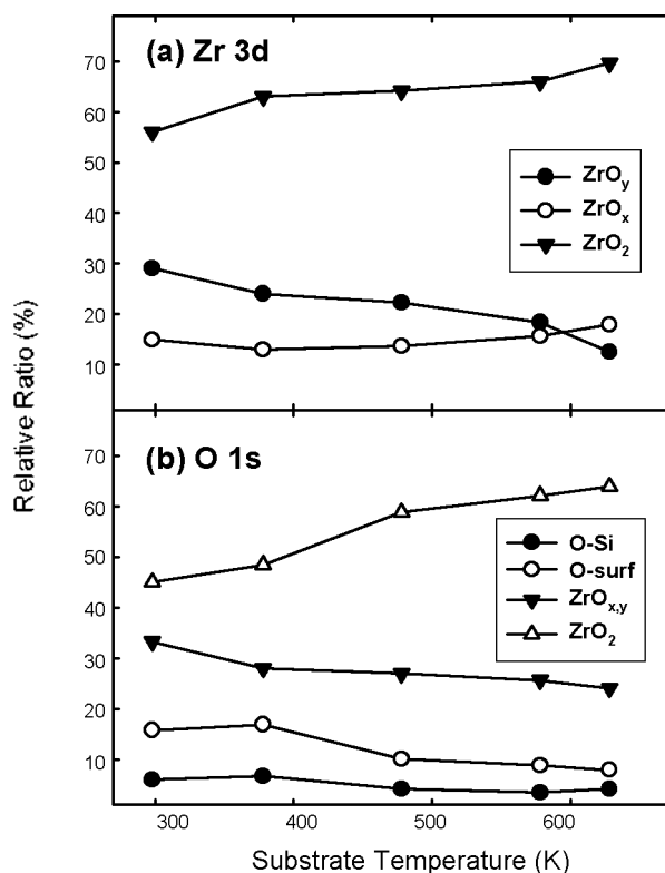
Figure 7. The relative peak area ratios of the Zr 3d (a) and O 1s (b) of the zirconium oxide thin films on Si(100) as a function of substrate temperatures.
