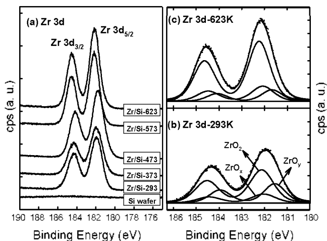
Figure 5. (a) stacked XP spectra of the Zr 3d 5/2 and 3d 3/2 of zirconium oxide thin films on Si(100) with increased substrate temperature. Deconvoluted XP spectra of the Zr 3d at the silicon substrate temperature of 293 K (b) and 623 K (c). The Zr 3d spectrum was decomposed three oxidation states: zirconia (ZrO 2 ), zirconium with higher (ZrO x ) and lower oxidation states (ZrO y ). The dots represent raw data, smooth lines overlapped with the dots represent reconstructed data of deconvoluted Zr 3d components.
