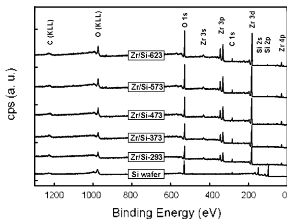
Figure 4. The survey XPS of zirconium oxide on Si(100) before and after zirconium oxide deposition with different substrate temperatures.
