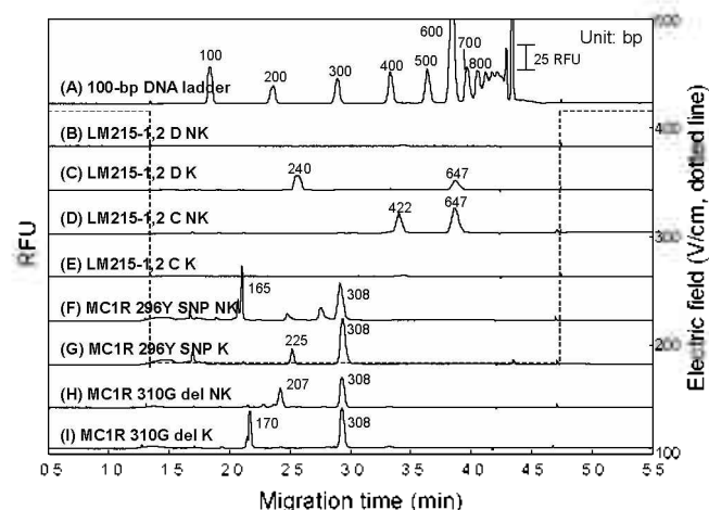
Figure 2. Representative electropherograms based on the voltage programming by CE-LIF of the various Korean cattle and non-Korean cattle SNP markers under the optimum separation conditions. CE separation conditions: sample separation electric field, 420 V/cm for 1.3 min, 180 V/cm for 2.9 min and 420 V/cm for 0.5 min. Indications: (A) = Standard 100-bp DNA ladder. (B) = LM215-1,2 D non-Korean cattle. (C) = LM215-1,2 D Korean cattle. (D) = LM215-1,2 C non-Korean cattle. (E) = LM215-1,2 C Korean cattle. (F) = MC1R 296Y SNP non-Korean cattle. (G) = MC1R 296Y SNP Korean cattle. (H) = MC1R 310G del non-Korean cattle. (I) = MC1R 310G del Korean cattle. The other CE conditions are the same as those shown in Figure 1.
