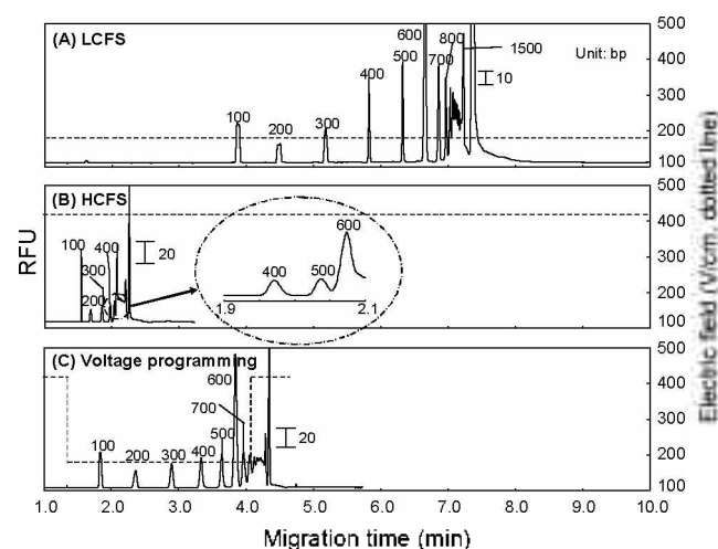
Figure 1. Comparisons of CE-LIF electropherograms for the 100-bp DNA ladder obtained using (A) LCFS, (B) HCFS, and (C) voltage programming. CE separation condition: Capillary, 75 \mu m I.D. fused-silica capillary; total length, 25 cm; effective length, 10 cm; excitation source, 5 mW He-Ne laser (543 nm); running buffer, 0.5 ppm EtBr in 1 \times TBE buffer (pH 8.45); coating gel, 1.0% PVP ( M_n 1,000,000); sieving matrix, 0.8% PEO ( M_n 8,000,000). 100-bp DNA ladder (Invitrogen) concentration, 25 ng/ \mu L. Sample injection, electrokinetic injection at electric field strength of 120 V/cm for 10 s. Sample separation electric field: LCFS = 180 V/cm. HCFS = 420 V/cm. Voltage programming = 420 V/cm for 1.3 min, 180 V/cm for 2.9 min and 420 V/cm for 0.5 min. Indications: LCFS, low constant field strength; HCFS, high constant field strength. The blue dotted line represents the applied electric field. RFU = relative fluorescence unit.
