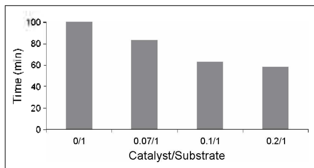
Figure 1. The catalyst amount effect on the conversion time of 1 mmol phenylacetic acid using 1.5 mmol (n\text{-Bu})_4\text{NIO}_4 and 40% molar ratio of imidazole. a ( a Based on disappearance and/or recovery of phenylacetic acid. For 0/1 catalyst to substrate after 100 minutes, the conversion was < 10%).
