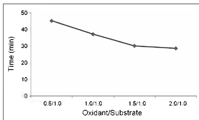
Figure 2. The oxidant amount effect on the conversion time of 1 mmol of phenylacetic acid using 10% and 40% molar ratio of catalyst and imidazole.
