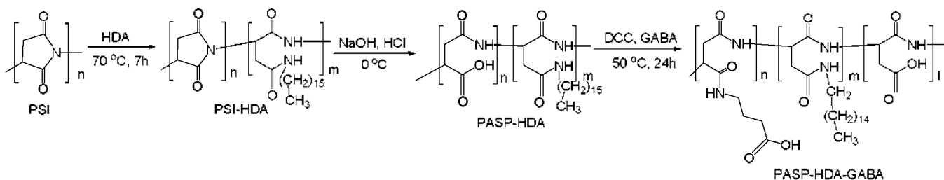
Scheme 2. Synthesis of GABA-conjugated amphiphilic polyaspartamides
