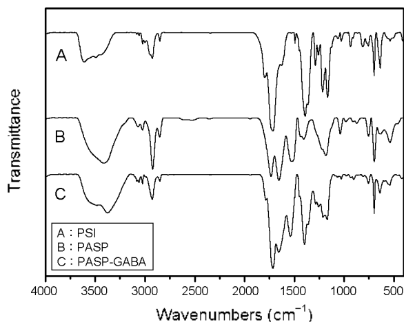
Figure 1. FT-IR spectra of PSI (A), PASP (B), and PASP-GABA (C).
