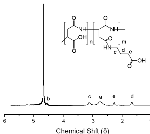
Figure 2. 1 H-NMR spectrum of PASP-GABA (D 2 O).
