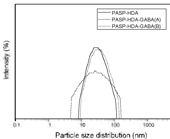
Figure 5. Particle size distributions of amphiphilic polyaspartamides in PBS (pH 7.4).
