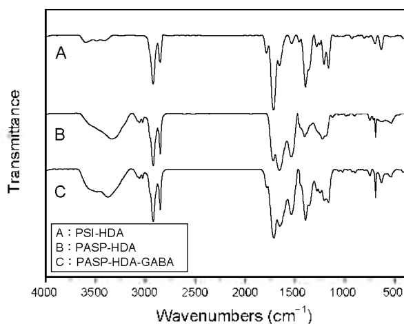
Figure 3. FT-IR spectra of PSI-HDA (A), PASP-HDA (B), PASP-HDA-GABA (C).
