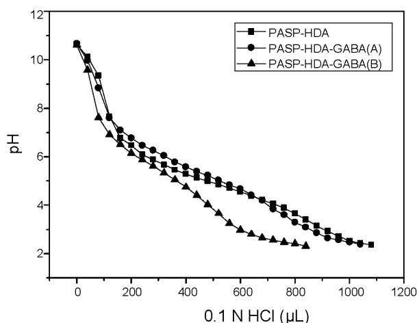
Figure 8. Acid-base titration profile of amphiphilic polyaspartamides.
