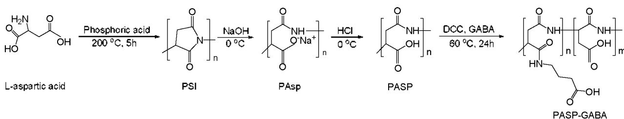
Scheme 1. Synthesis of GABA-conjugated PASP (PASP-GABA)
