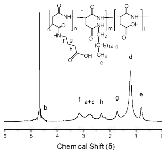
Figure 4. ^1\text{H-NMR} spectrum of PASP-HDA-GABA ( \text{D}_2\text{O} ).
