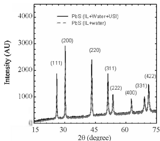
Figure 1. The powder XRD pattern of as-prepared PbS nanoclusters prepared in ionic liquid and water (1:1 in volume) with and without the aid of USI.
