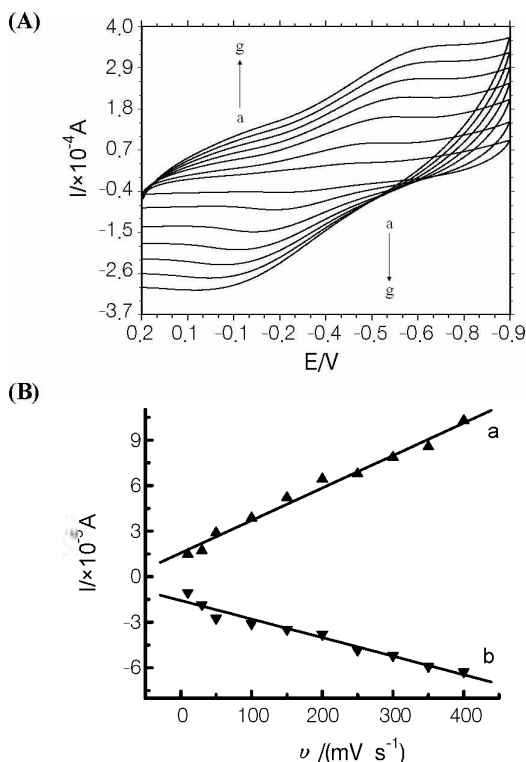
Figure 5. (A) Cyclic voltammograms of the CTS/nano-TiO 2 /Hb/CILE in pH 7.0 PBS at the scan rate of 10, 50, 100, 150, 200, 250, 300 mV s -1 (from a to g). (B) The linear relationships of the cathodic (a) and anodic (b) peak current ( I p ) versus the scan rate ( v ) in pH 7.0 PBS.
