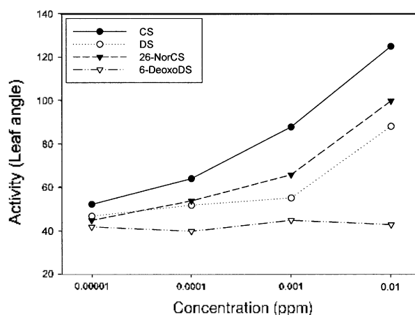
Figure 3. Biological activity for CS, DS, 6-deoxoDS and 26-norCS in the rice lamina inclination assay.
