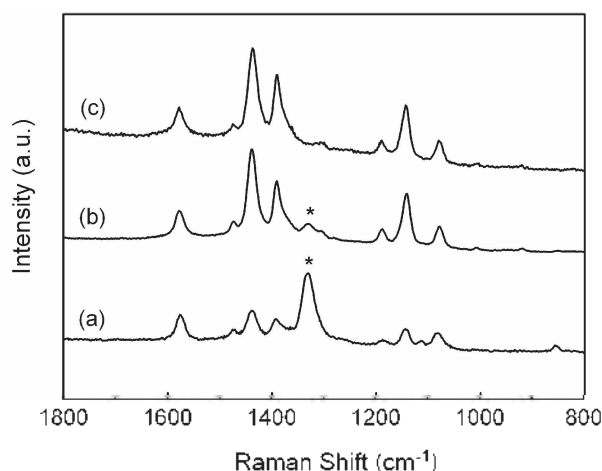
Figure 2. SERS spectra of bis(4-nitrophenyl) disulfide adsorbed on HNO 3 -etched Cu measured using (a) a slightly defocused and (b) a focused laser beam. (c) SERS spectrum of 4-aminobenzenethiol adsorbed on HNO 3 -etched Cu for comparison. All spectra were obtained using an Ar + laser at 514.5 nm as the excitation source. The stars (*) indicate the \nu_s(\text{NO}_2) peak.
