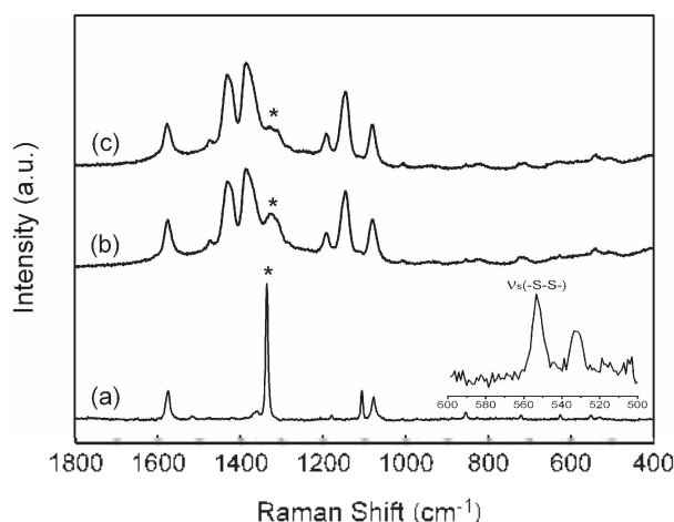
Figure 1. (a) Normal Raman spectrum of bis(4-nitrophenyl) disulfide in neat solid state. SERS spectra of bis(4-nitrophenyl) disulfide adsorbed on HNO 3 -etched Cu (b) measured immediately and (c) after 5 min. All spectra were obtained using a He/Ne laser at 632.8 nm as the excitation source. The stars (*) indicate the \nu_s(\text{NO}_2) peak. The inset spectrum shows the S-S stretching peak of pure bis(4-nitrophenyl) disulfide.
