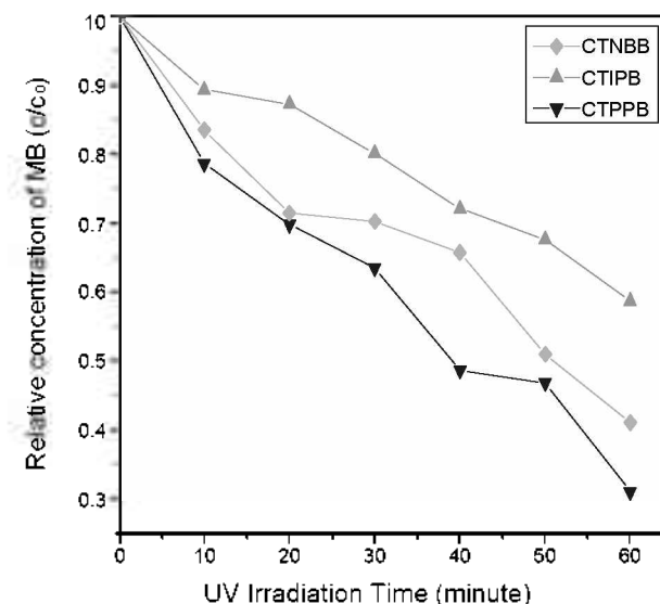
Figure 5. Dependence of relative concentration of MB in the aqueous solution c/c_0 on time of UV irradiation for the MWCNT/TiO 2 composites; the concentration of MB solution: 1.0 \times 10^{-5} mol/L.
