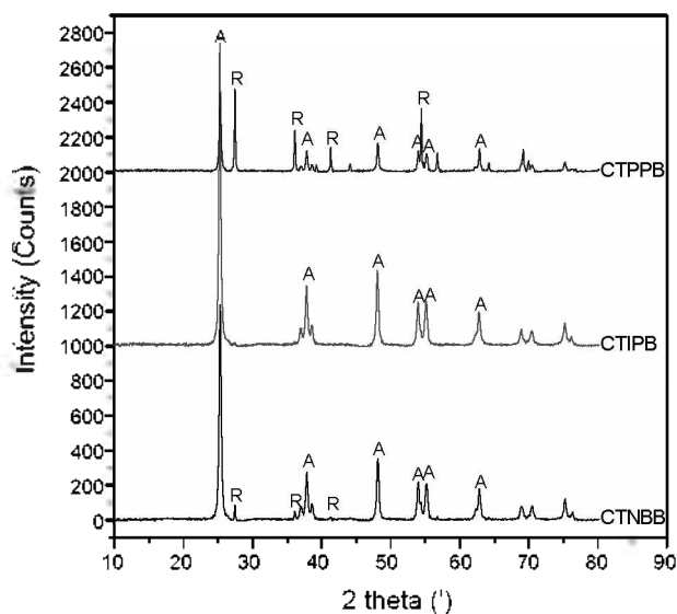
Figure 3. XRD patterns of the MWCNT/TiO 2 composites.
