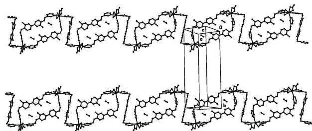
Figure 4. Packing diagram of a 1-D polymer 2 .
