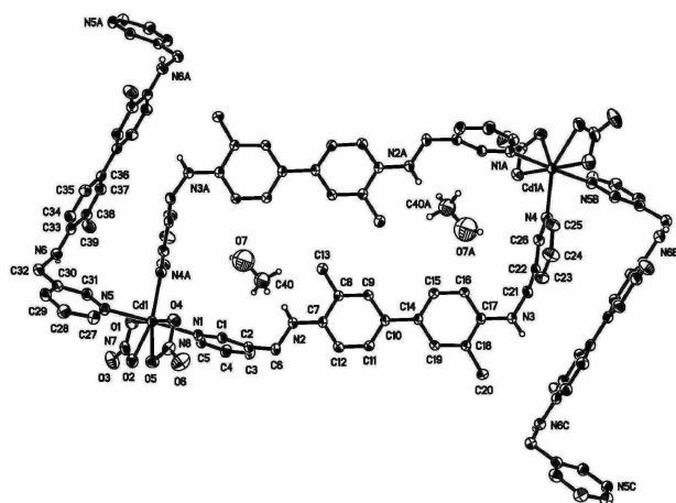
Figure 3. Local coordination environment around Cd in polymer 2 , with 30% probability thermal ellipsoids. Selected bond lengths (Å) and angles (°): Cd1-N5 2.293(2), Cd1-N1 2.320(2), Cd1-N4#1 2.338(2), Cd1-O2 2.364(2), Cd1-O5 2.446(2), Cd1-O4 2.488(2), Cd1-O1 2.551(2), N2-C7 1.376(3), N2-C6 1.433(4), N3-C17 1.390(3), N3-C21 1.452(4), N6-C33 1.369(4), N6-C32 1.440(4), N5-Cd1-N1 176.96(8), N5-Cd1-N4#1 90.10(8), N1-Cd1-N4#1 92.55(8). Symmetry transformations used to generate equivalent atoms: #1 = -x, -y, -z + 1.
