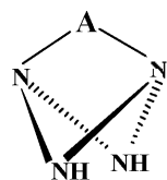
Figure 5. The tetrahedrally tilted pyrrolenine nitrogens of a porphyrin core: two nitrogen atoms of pyrrolenine in one side of the porphyrin plane act as the electron donors to the acceptor (A: \text{ZrO}(\text{NO}_3)_2 ).
