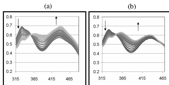
Figure 1. Family of spectra recorded over the course of titration of 30 μM acetonitrile solution of the receptor 1 with a standard solution tetrabutylammonium fluoride (a) and acetate (b).
