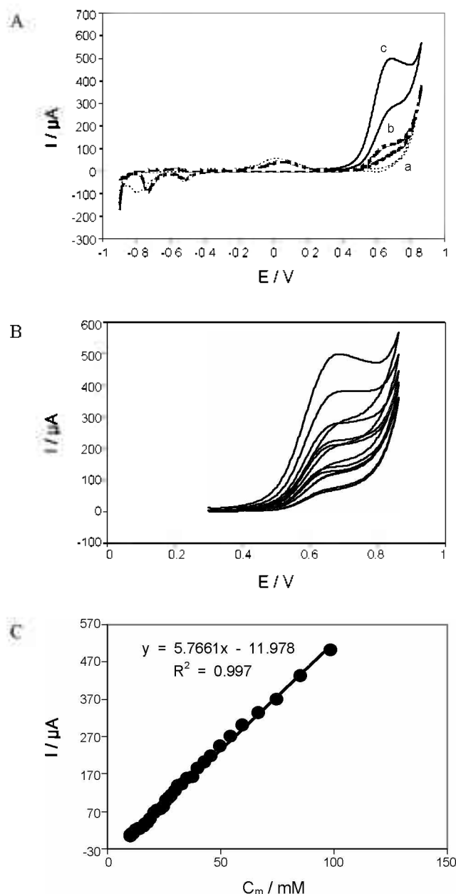
Figure 2. A: Cyclic voltammograms (CVs) of Cu electrode (b) and Cu/CuDMG electrode (c) in the absence (a) and the presence (b and c) of 0.2 M cyclohexanol in 0.1 M NaOH solution at a potential sweep rate of 10 mV/s. B: Cyclic voltammograms of Cu/CuDMG electrode in 0.1 M NaOH solution in the presence of different concentrations of cyclohexanol in Cu/CuDMG electrode. From inner to the outer: 0.03 (a) 0.08 (b), 0.1 (c), 0.15 (d), 0.2 (e), and 0.25 M (f), respectively. The potential sweep rate is 10 mV/s. C: Dependency of peak current on the concentration of cyclohexanol in the range of 0.01 - 0.1 M.
