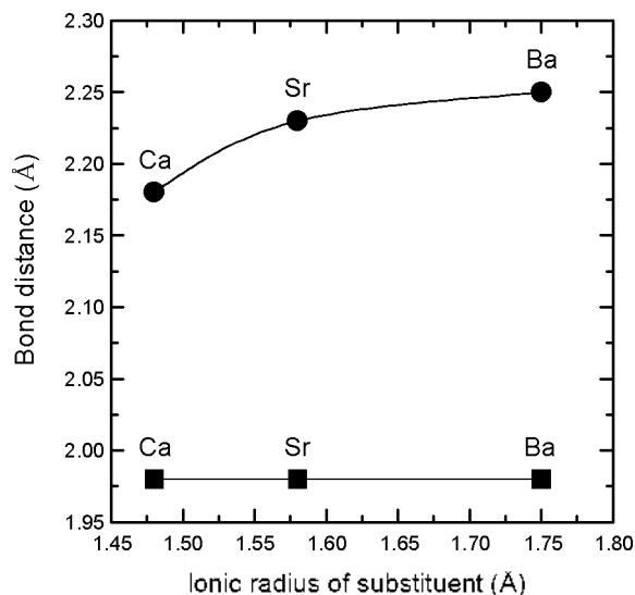
Figure 4. Dependences of axial bond distances of (\text{Cu}-\text{O}_{\text{Sr}}) and (\text{Ru}-\text{O}_{\text{Sr}}) on the ionic size of substituent alkali metal ions in \text{RuSr}_{1.9}\text{A}_{0.1}\text{GdCu}_2\text{O}_8 (A = Ca, Sr, and Ba). The circles and squares represent the bond distances of (\text{Cu}-\text{O}_{\text{Sr}}) and (\text{Ru}-\text{O}_{\text{Sr}}) , respectively.
