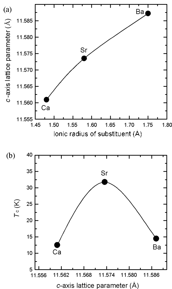
Figure 2. Dependences of (a) c -axis lattice parameter and (b) T_c on the ionic size of substituted alkali metal ions in \text{RuSr}_{1.9}\text{A}_{0.1}\text{GdCu}_2\text{O}_8 ( \text{A} = \text{Ca}, \text{Sr}, \text{and Ba} ).
