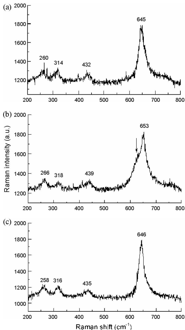
Figure 3. Micro-Raman spectra for the alkaline earth metal-substituted \text{RuSr}_{1.9}\text{A}_{0.1}\text{GdCu}_2\text{O}_8 with A = (a) Ca, (b) Sr, and (c) Ba. In (b), the arrow denotes the low energy shoulder peak of \text{O}_{\text{Sr}} vibration mode.
