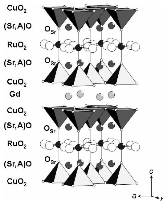
Figure 1. Crystal structure of the alkaline earth metal-substituted \text{RuSr}_{1.9}\text{A}_{0.1}\text{GdCu}_2\text{O}_8 ( \text{A} = \text{Ca}, \text{Sr}, \text{and Ba} ).
