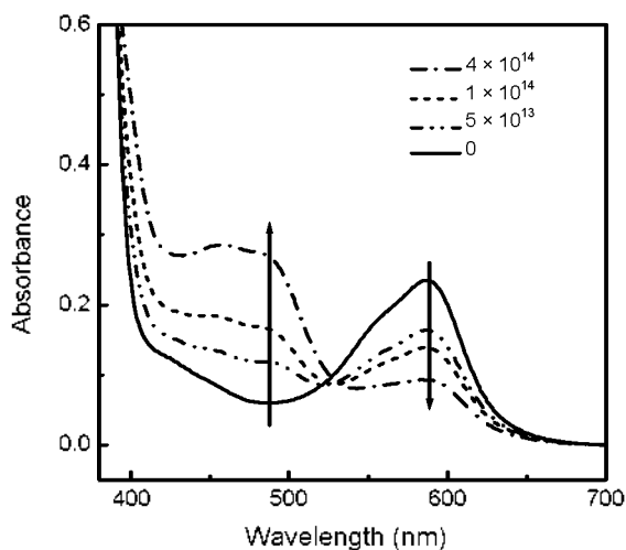
Figure 2. Effects of proton fluence on the spectra of SPO/PS. The ion energy was 25 MeV and the numbers in the figure indicate ion fluence in the unit of \text{ions}/\text{cm}^2 .
