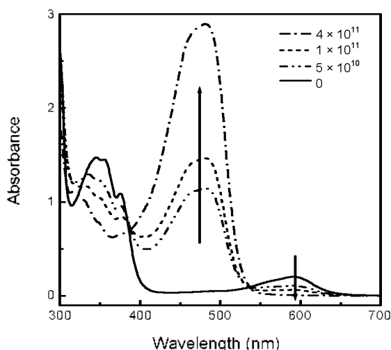
Figure 1. Effects of proton fluence on the spectra of SPO/ \text{CHCl}_3 . The ion energy was 25 MeV and the numbers in the figure indicate ion fluence in the unit of \text{ions}/\text{cm}^2 .
