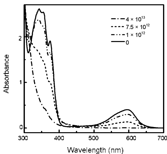
Figure 3. Effects of proton fluence on the spectra of SPO/ethanol. The ion energy was 25 MeV and the numbers in the figure indicate ion fluence in the unit of \text{ions}/\text{cm}^2 .
