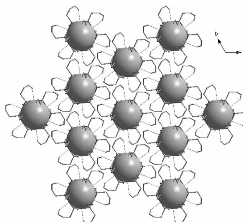
Figure 4. Packing diagram of \beta form (the dashed are the bonds of Ni-H)
