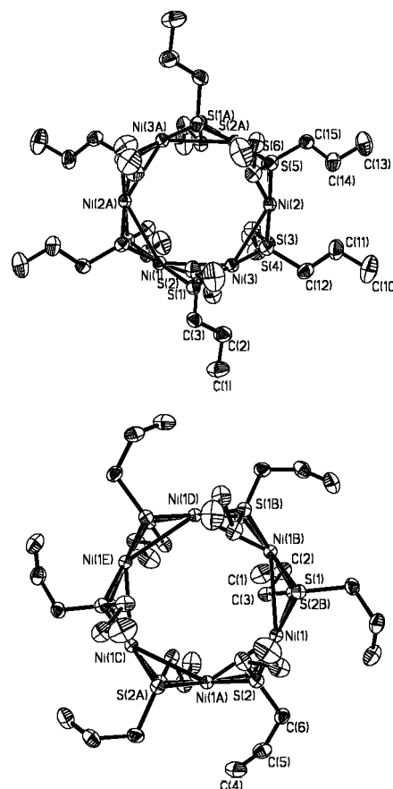
Figure 1. Molecular structure for \alpha (up) and \beta -form (down) along with atom labeling. The crystal of \alpha form is in triclinic crystal system with P\bar{1} space group and the crystal of \beta form is in trigonal crystal system with R\bar{3} space group.
