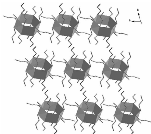
Figure 3. Packing diagram of \alpha form.
