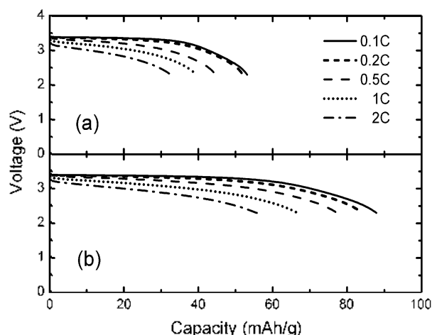
Figure 8. The discharge voltage profiles for the electrodes as a function of the specific capacity for (a) \text{LiFePO}_4 powder and (b) the chitosan added \text{LiFePO}_4 powder. In both cases, the charge rate was 0.2 C and discharge rates were different.
