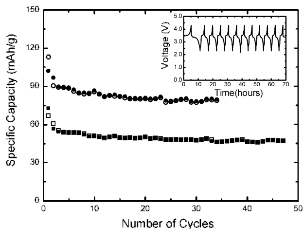
Figure 7. The specific capacity upon discharge rate of 0.2 C with the number of cycles. The squares and circles represent \text{LiFePO}_4 powder after the second calcination and the chitosan added \text{LiFePO}_4 powder after the third calcination, respectively. Open and solid points represent charging and discharging processes, respectively. The inset shows the charge-discharge cycles of the \text{LiFePO}_4 electrodes. The potential range was between 2.5 V and 4.3 V.
