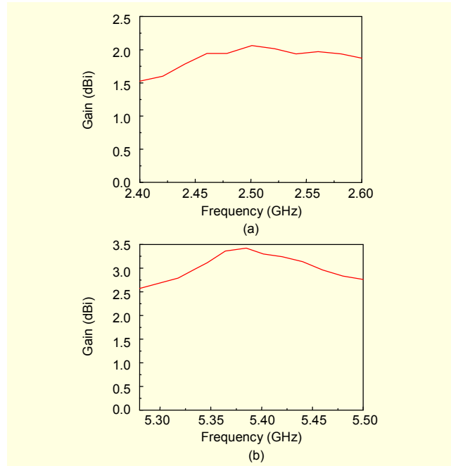
Fig. 8. Measured gain of the antenna: (a) at lower band and (b) at upper band.
