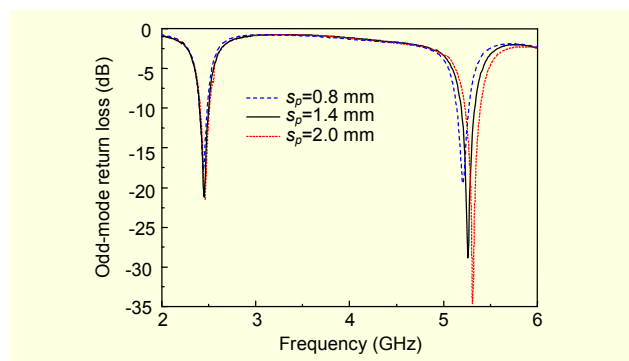
Fig. 5. Simulated effect of patch spacing on odd-mode return loss.
