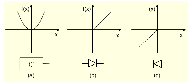
Fig. 5. Transfer functions of nonlinear processing: (a) x^2 , (b) D(x) , and (c) RD(x) .
