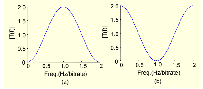
Fig. 4. Transfer functions of the spectrum processing: (a) r(t)-r(t-T/2) and (b) r(t)+r(t-T/2) .
