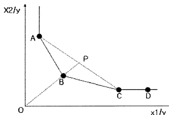
Fig. 1. Super-efficiency example.
