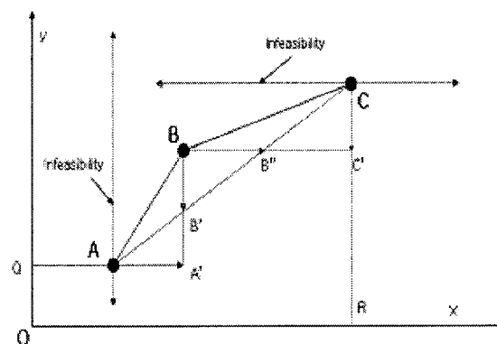
Fig. 2. Infeasibility example.
