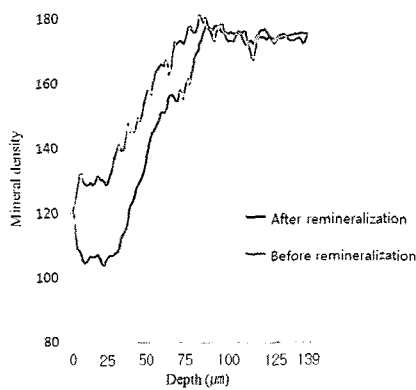
Figure 10. Comparison of density in enamel area before and after remineralization (Group 1).
