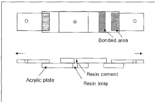
Figure 1. Diagram of the prepared specimens.
