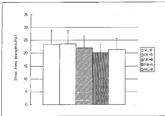
Figure 4. Shear bond strength of the five resin cements to indirect resin restorations treated with silane and adhesives or primers.
