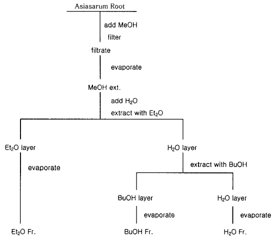
Scheme 1. Fractionation of Asiasarum Root.
