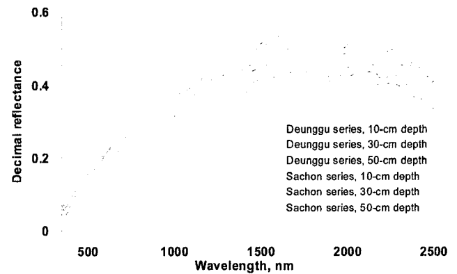
Fig. 1 Soil reflectance spectra for two soil series at three depths.
