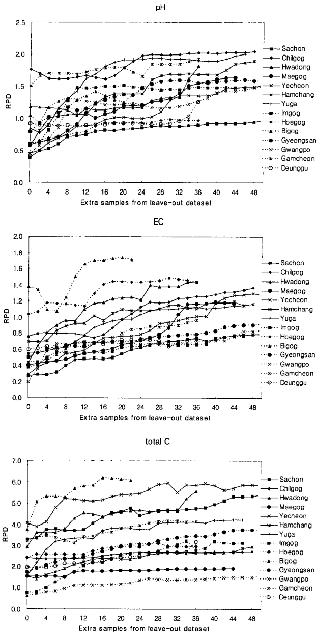
Fig. 3 RPD of calibration model vs. number of sample points included from the “leave-out” dataset for pH (top), EC (middle), and total C (bottom).
