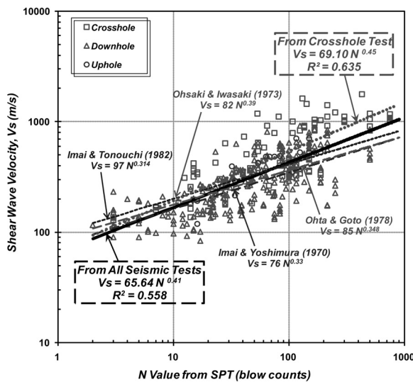
〈Figure 4〉 Correlation between V_S and Measured N Value for All Soils in Korea
