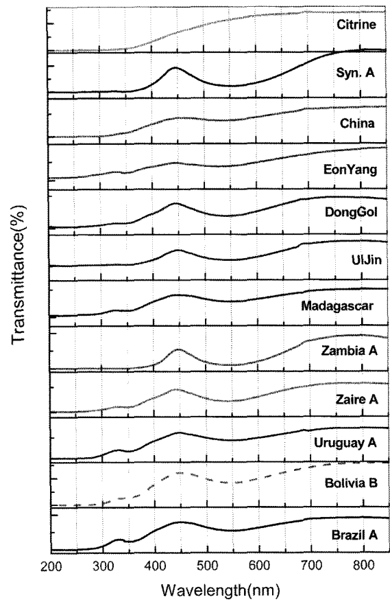
Fig. 4. UV-VIS transmission pattern of amethyst from various origin.
