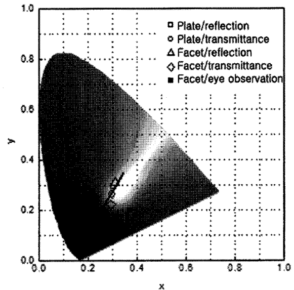
Fig. 6. Chromaticity values of Uljin amethysts plotted on CIE xyY color space.
