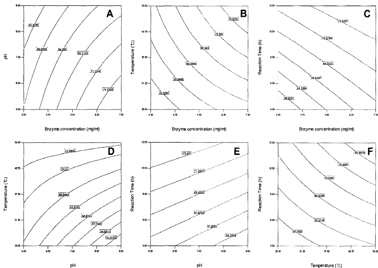
Fig. 4. Contour plots between any two factors for yield of icariside II: Other two factors were kept at the central point.
