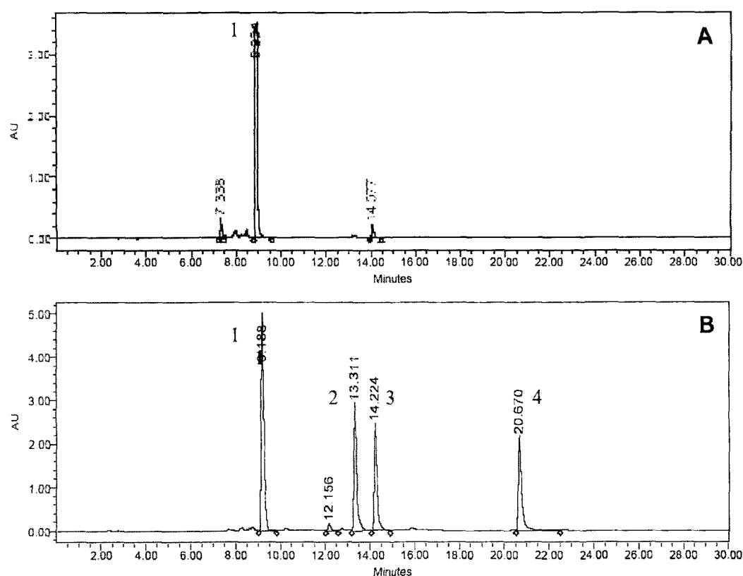
Fig. 1. HPLC profiles of icariin from Epimedium grandiflorum (A) and partial acid hydrolysate of icariin (B). Key to peak identity: 1, icariin; 2, compound 1; 3, compound 2; 4, compound 3.
