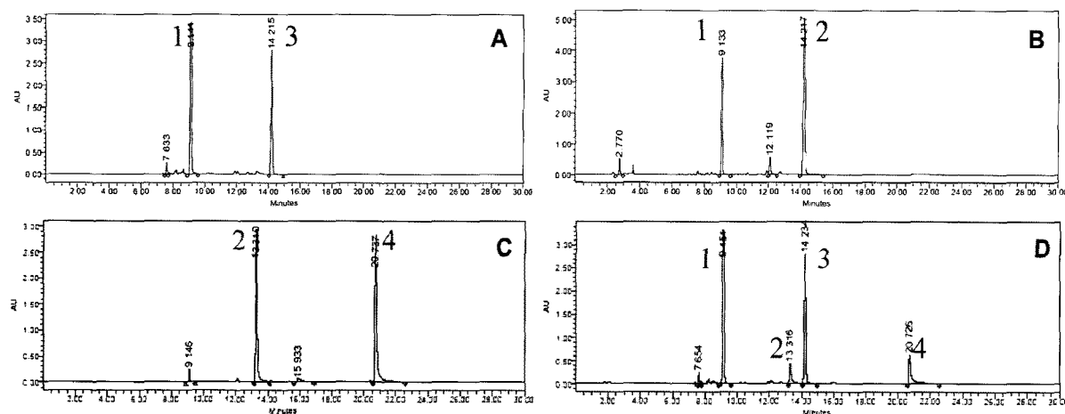
Fig. 3. HPLC profile of hydrolysate of icariin using several glycolytic enzymes; reaction with beta-glucosidase (A), cellulase (B), naringinase (C), and hesperidinase (D).
