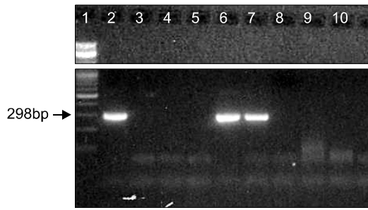
Figure 1. The Result of CMV-PCR. 1: molecular marker; 2: positive control; 3~5: negative control; 6: patient blood sample; 7: patient BAL sample; 8~10: negative control.
