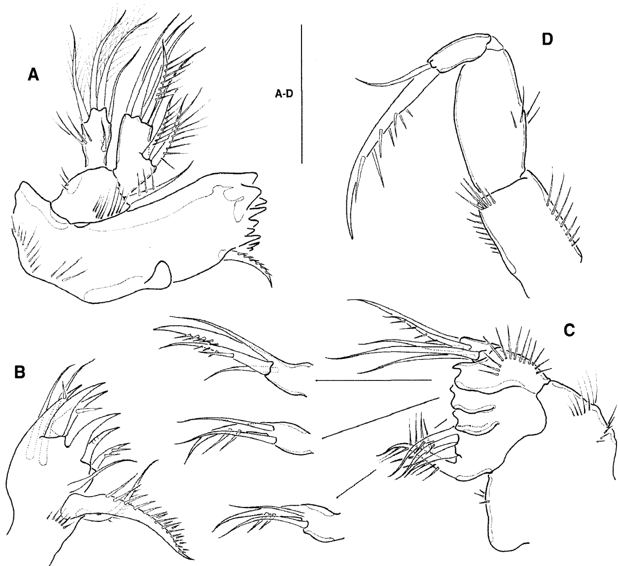
Fig. 4. Microarthridion litospinatus Shen and Tai, male. A, mandible; B, praecoaxal arthrite of maxillule; C, maxilla; D, maxilliped. Scale bar=20 \mu m.
