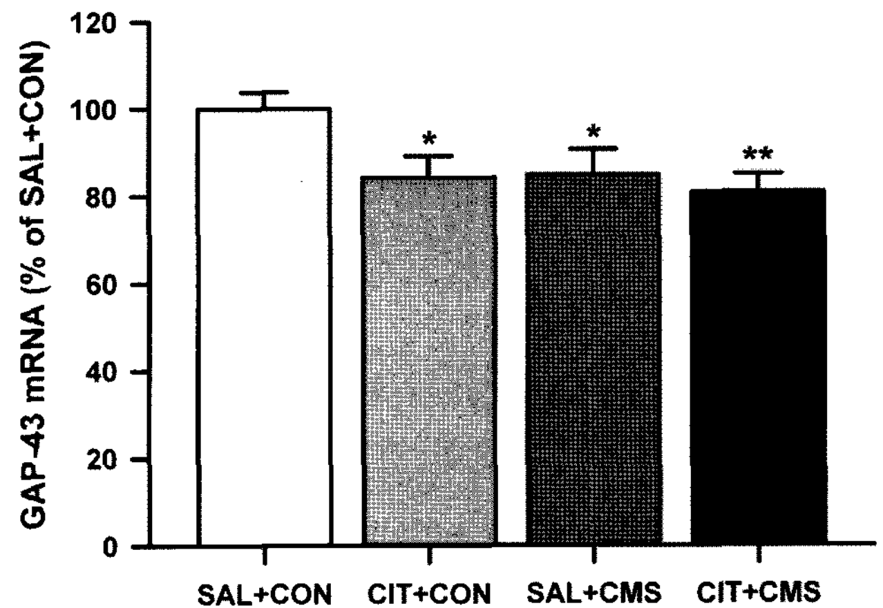
Fig. 3. The effects of repeated citalopram treatment and CMS on GAP-43 mRNA levels in the GCL. Repeated citalopram treatment and CMS significantly decreased GAP-43 mRNA levels in the GCL, but there was no significant interaction between repeated citalopram treatment and CMS. The results are expressed as percent of mean value from SAL+CON group and are mean±S.E.M (n=9 per group). Data were compared using a one-way ANOVA with Fisher's LSD post hoc test. * p<0.05 and ** p<0.01 vs. saline-treated unstressed control (SAL+CON). Abbreviations used: citalopram treated unstressed group (CON+CIT), saline treated CMS-exposed group (CMS+SAL), citalopram treated CMS-exposed group (CMS+CIT).
