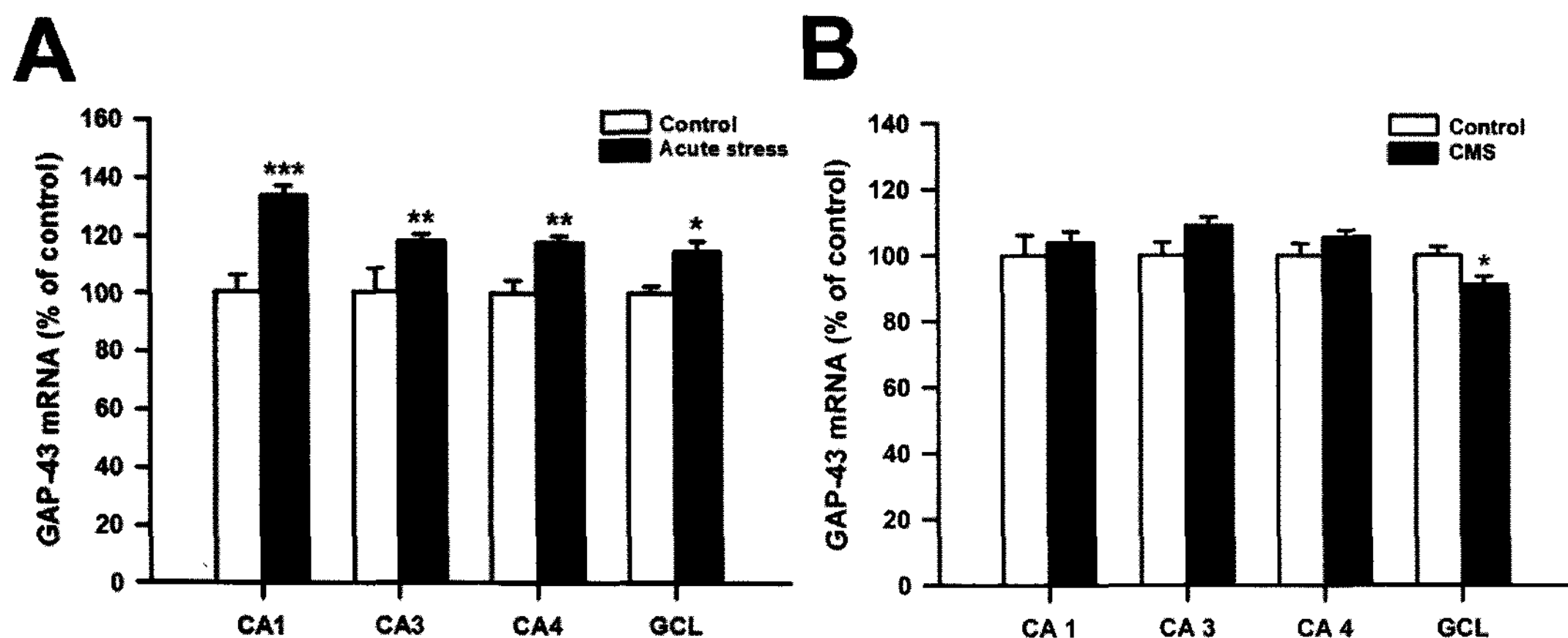
Fig. 1. (A) The effects of acute stress on GAP-43 mRNA levels in CA1, CA3, CA4 and dentate granular cell layer (GCL) of the hippocampus (n=4 per group) (B) The effects of chronic mild stress (CMS) on GAP-43 mRNA levels in the CA1, CA3, CA4 and GCL of the hippocampus (n=7 per group). The results are expressed as percent of mean value from control group and are mean standard error of mean (S.E.M.). Data were compared by Student's t -test. * p < 0.05 , ** p < 0.01 and *** p < 0.001 vs. control group.
