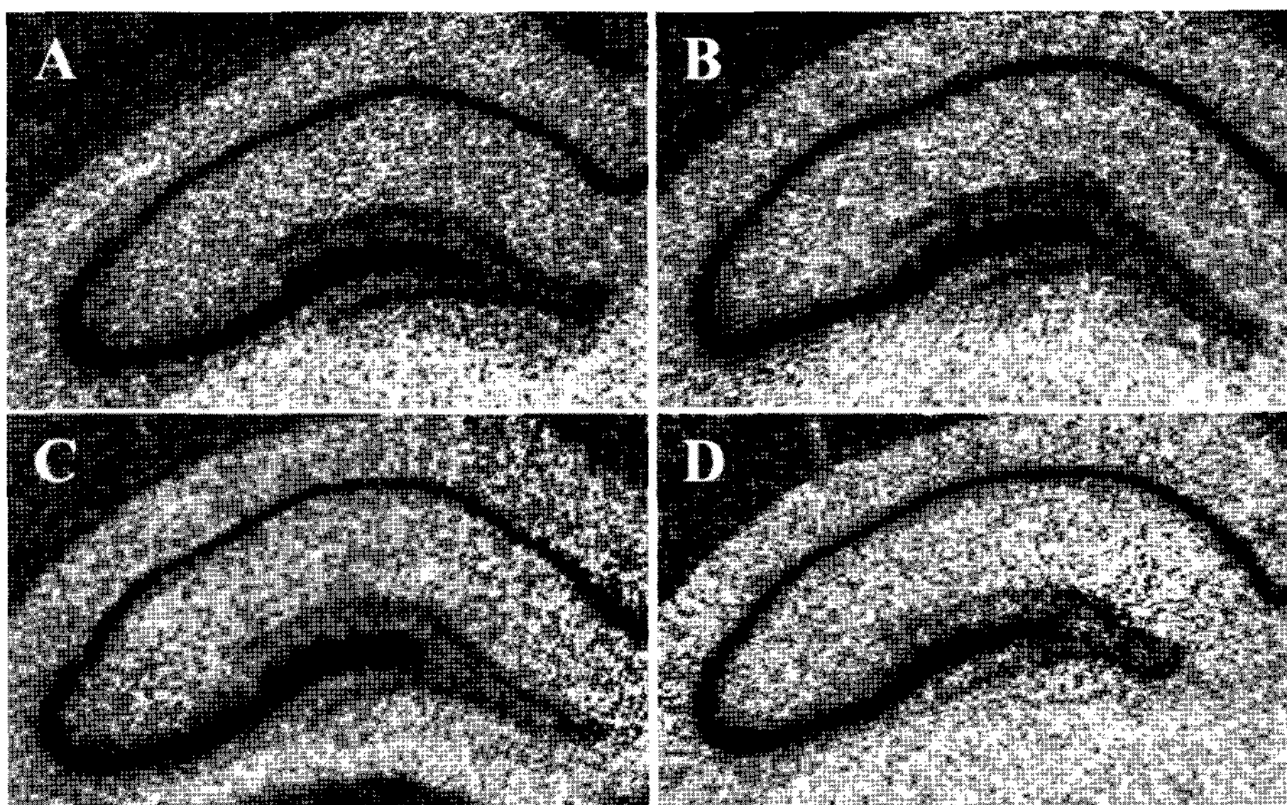
Fig. 4. Representative autoradiographs of ^{35}\text{S} -labeled GAP-43 mRNA in the hippocampus from each treatment group are shown. (A) saline treated unstressed group (B) citalopram treated unstressed group (C) saline treated CMS-exposed group (D) citalopram treated CMS-exposed group.
