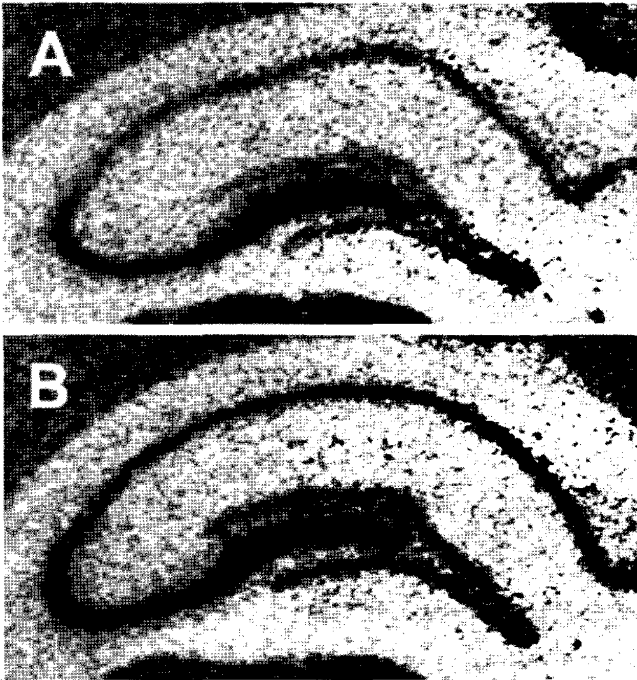
Fig. 2. Representative autoradiographs of ^{35}\text{S} -labeled GAP-43 mRNA expression in the hippocampus from each treatment group are shown. (A) control (B) acute immobilization stress.
