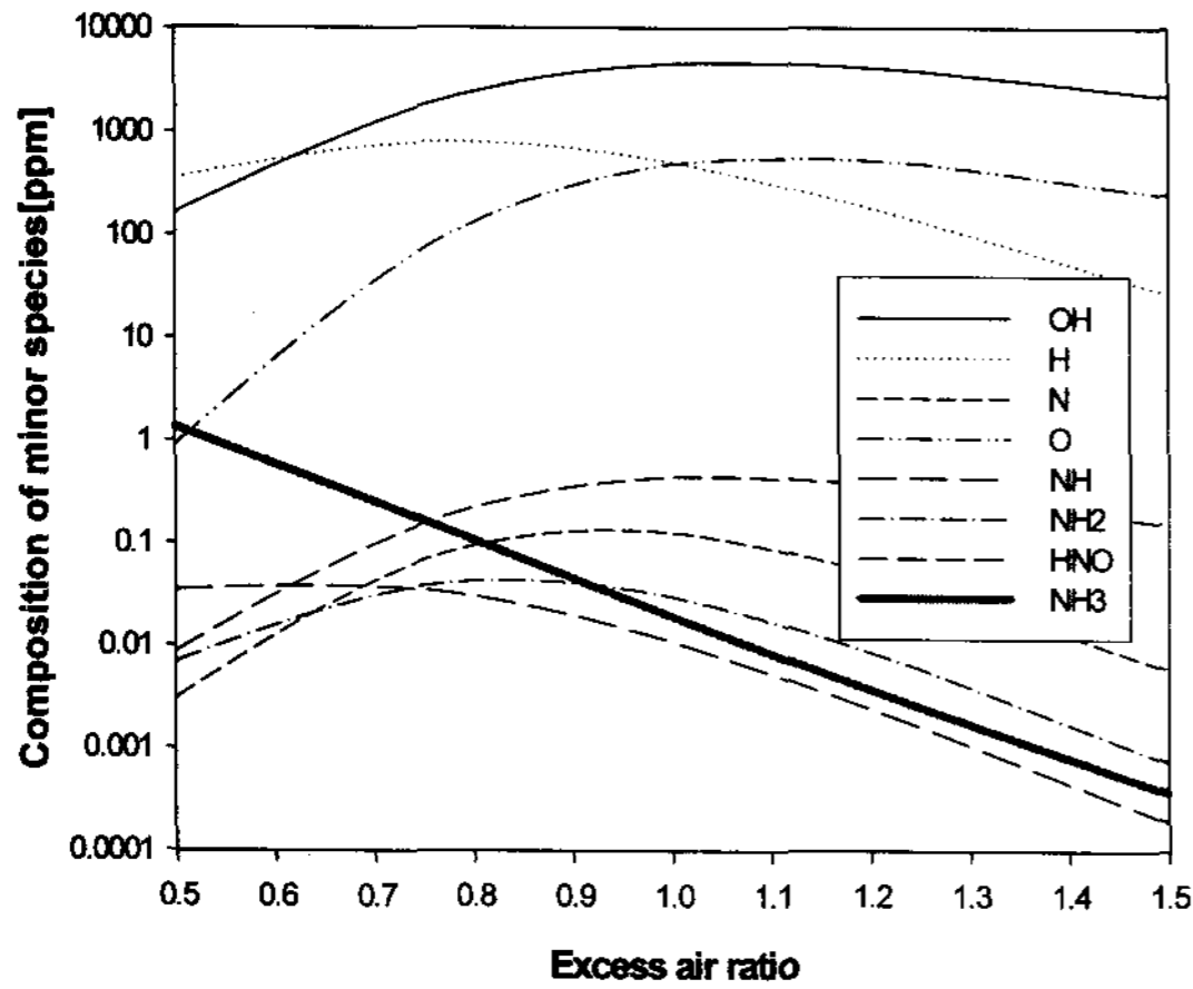
Figure 10. Composition of minor species (Syngas #3).
