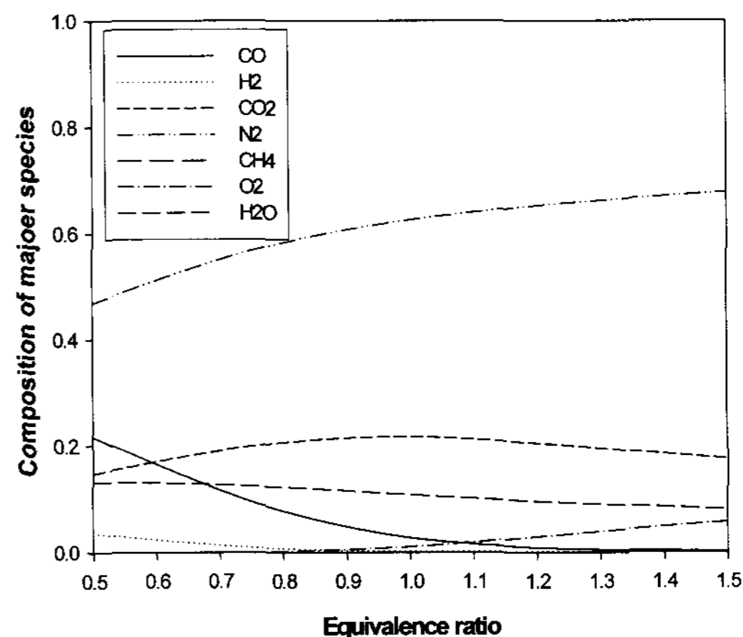
Figure 4. Composition of major species (Syngas #1).
