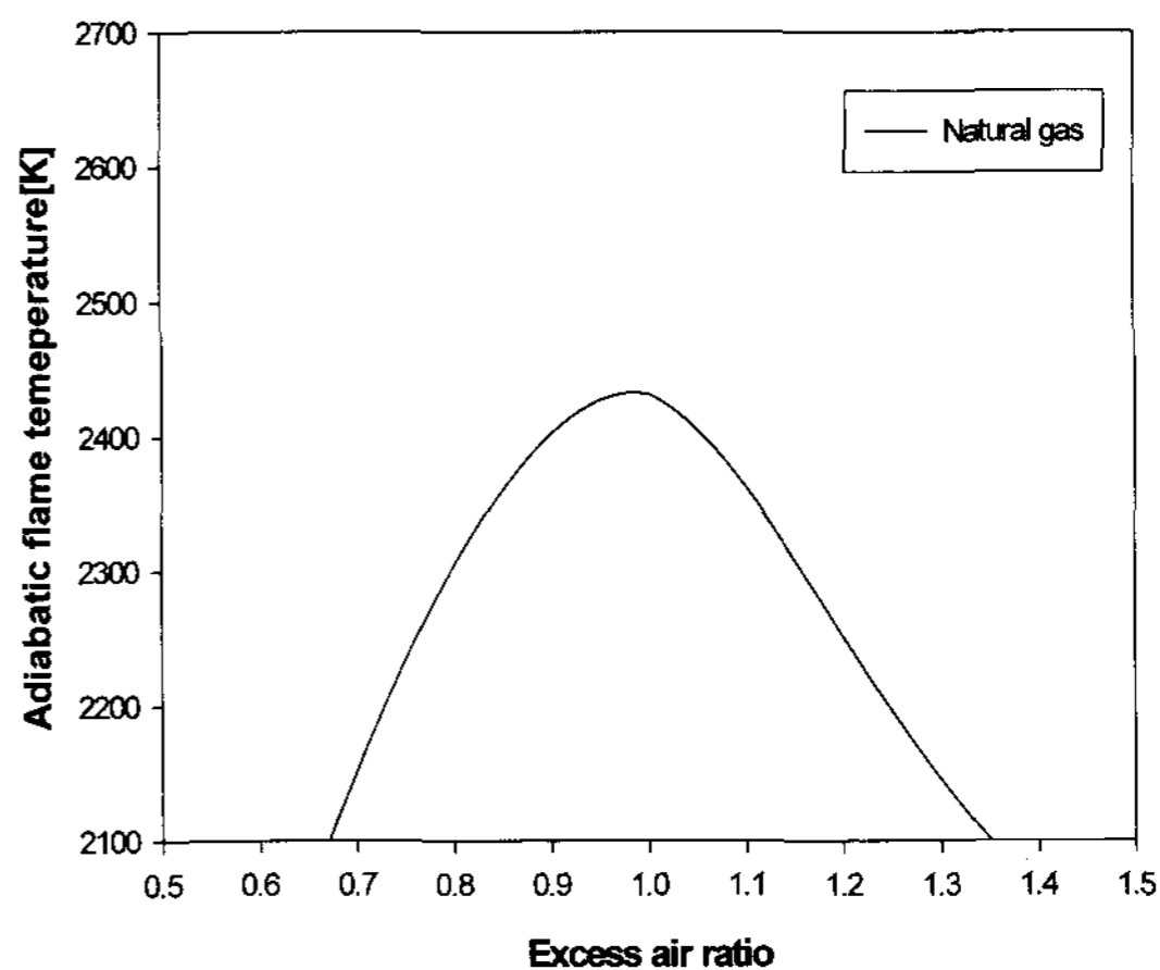
Figure 3. Flame temperature of natural gas.
