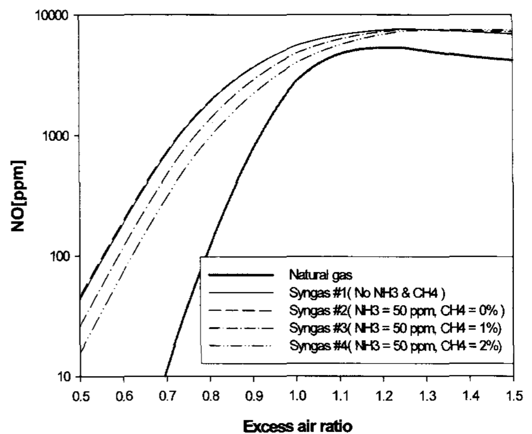
Figure 13. NOx emission from syngas fuel.
