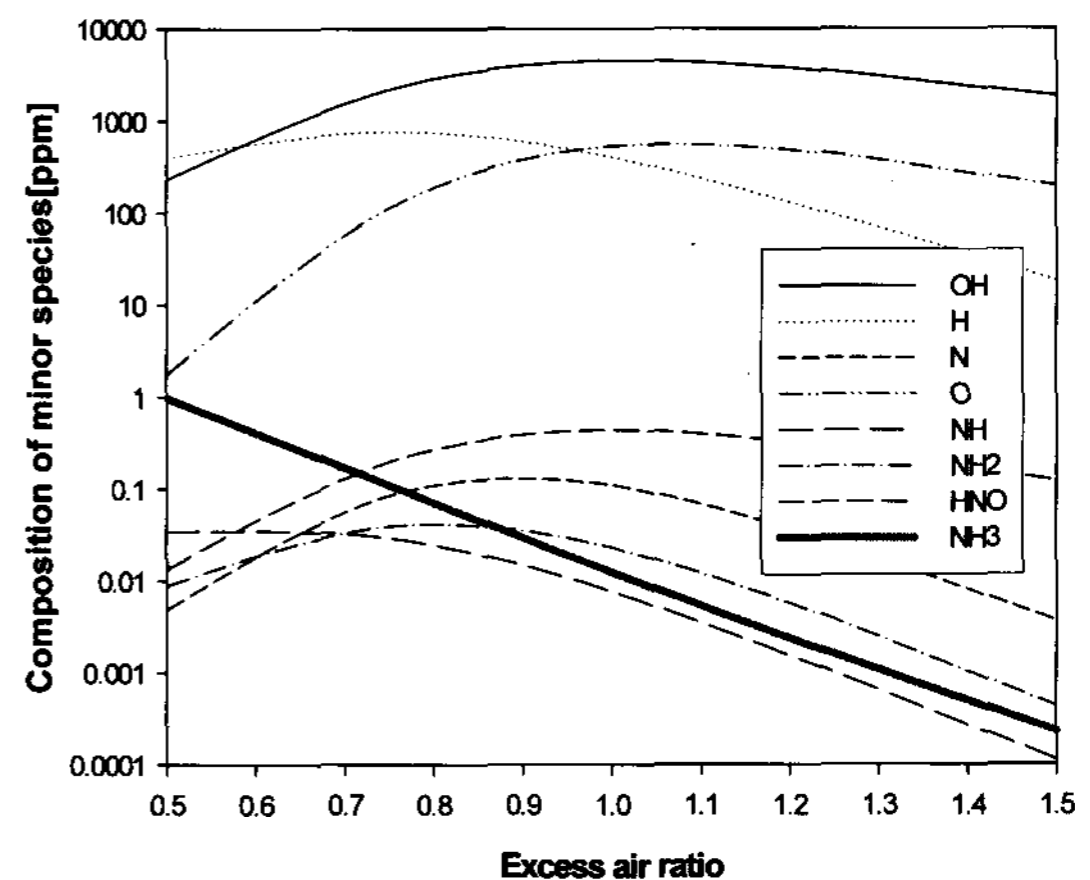
Figure 9. Composition of minor species (Syngas #2).
