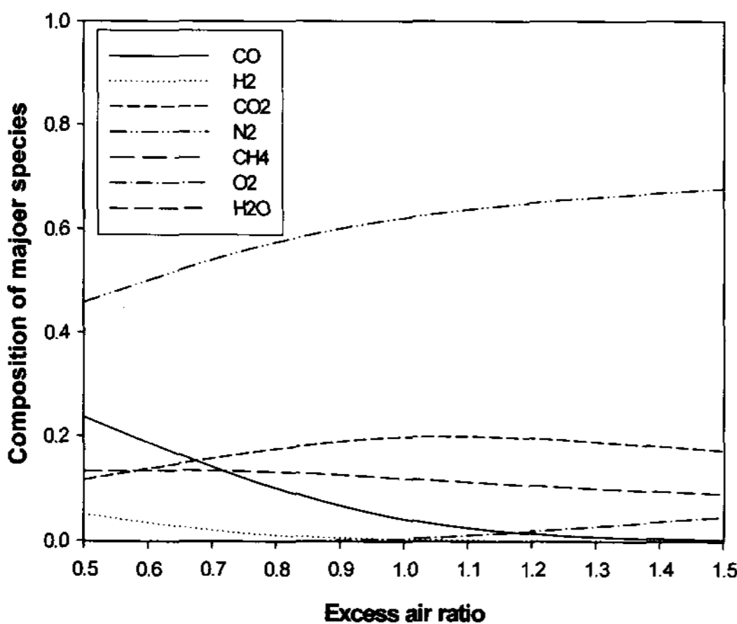
Figure 7. Composition of major species (Syngas #4).
