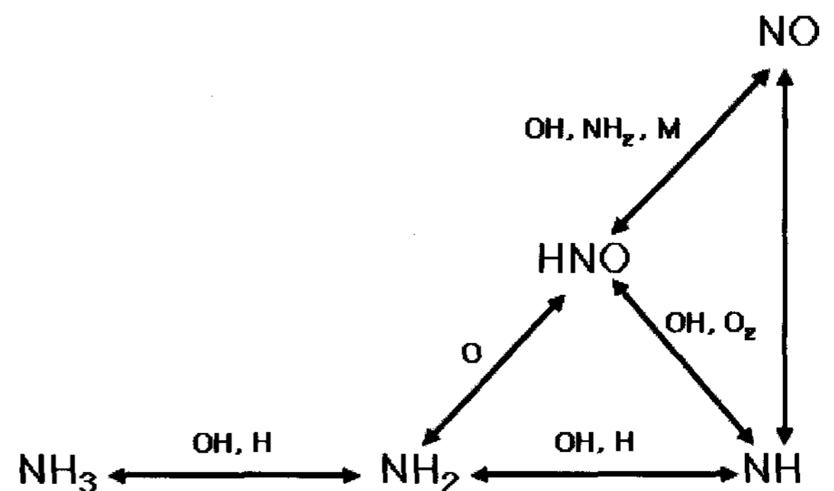
Figure 1. Fuel NO x formation mechanism and paths.
