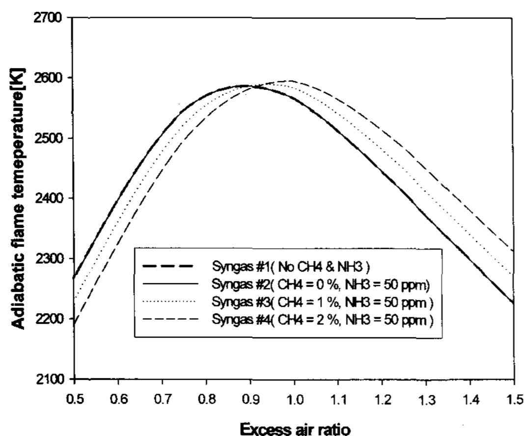
Figure 2. Flame temperature of syngas.
