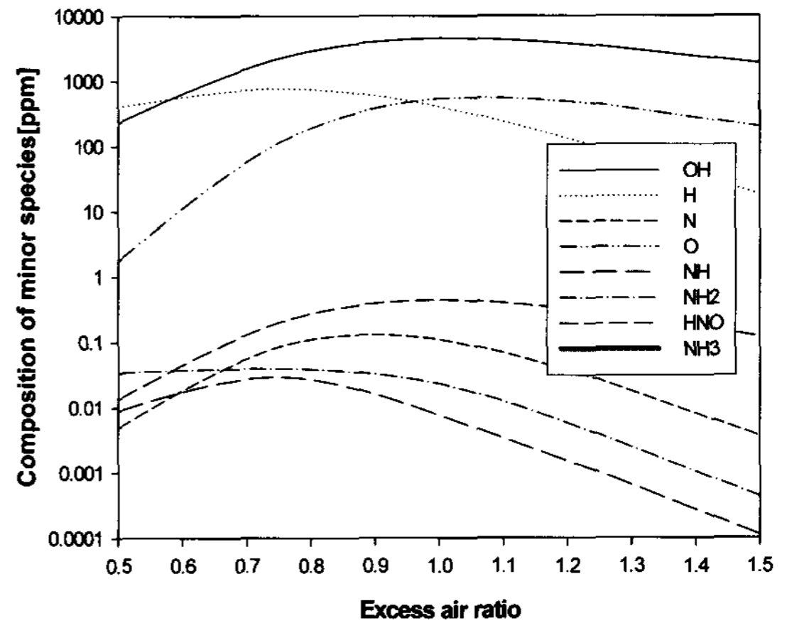
Figure 8. Composition of minor species (Syngas #1).
