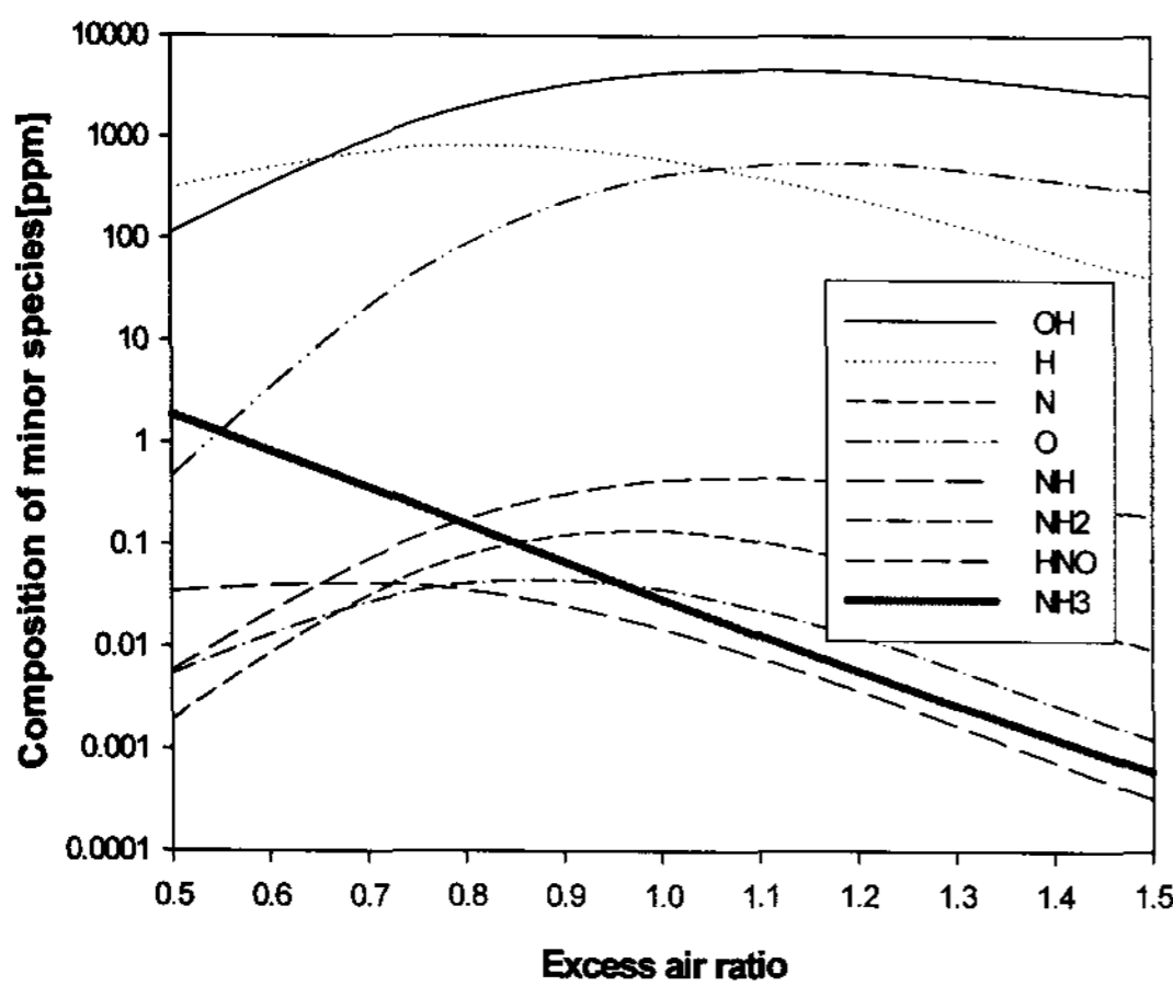
Figure 11. Composition of minor species (Syngas #4).
