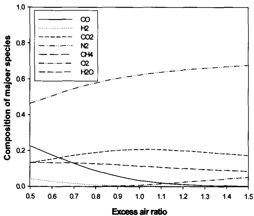
Figure 6. Composition of major species (Syngas #3).
