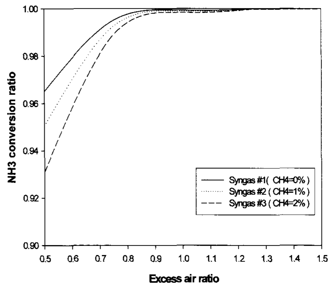
Figure 12. NH3 conversion ratio of syngas fuel.
