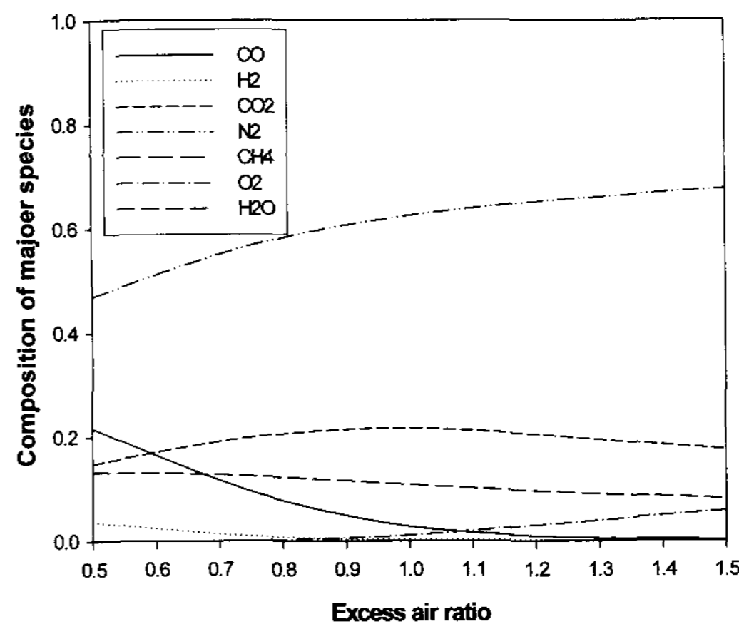
Figure 5. Composition of major species (Syngas #2).
